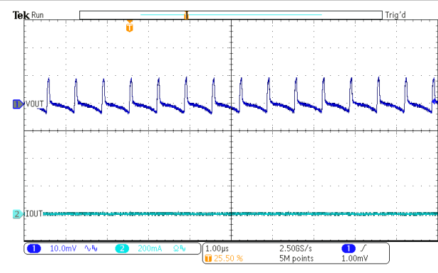
V_{IN} = 12\text{ V} I_{OUT} = 0\text{ A} Figure 7-15. Output Ripple – No Load
