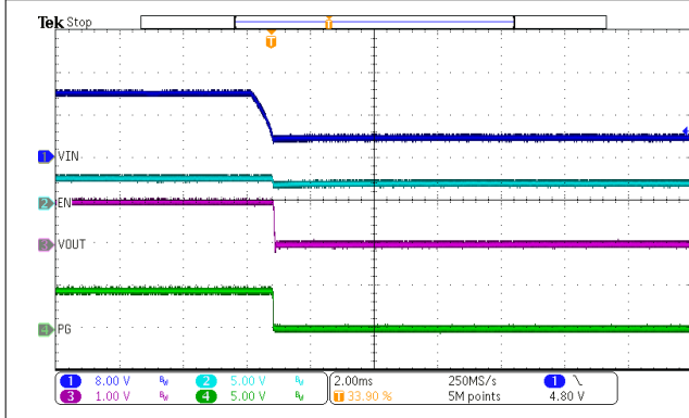
I_{OUT} = 8\text{ A} Figure 7-14. VIN Shutdown
