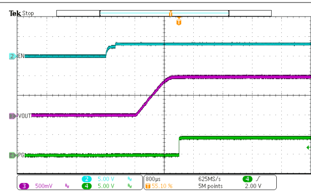
V_{IN} = 12\text{ V} I_{OUT} = 8\text{ A} Figure 7-11. EN Start-Up – With Load
