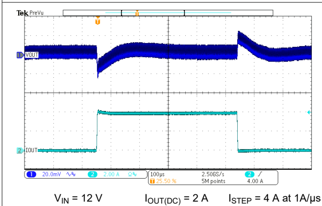
Figure 7-8. Load Transient
