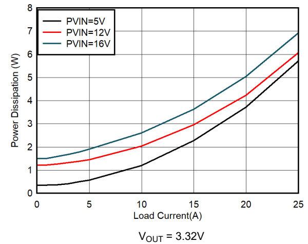
Figure 8-4. Power Dissipation
