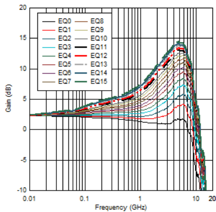
Figure 5-3. USB RX1 EQ Settings Curves
