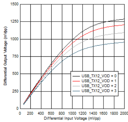
Figure 5-21. USB TX1 VOD Linearity Settings at 5GHz
