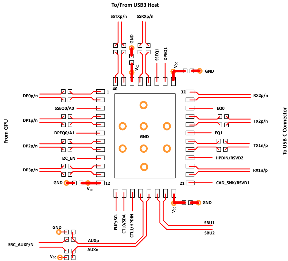
Figure 8-10. Layout Example
