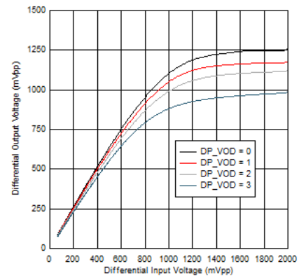
Figure 5-16. DP VOD Linearity Settings at 100MHz
