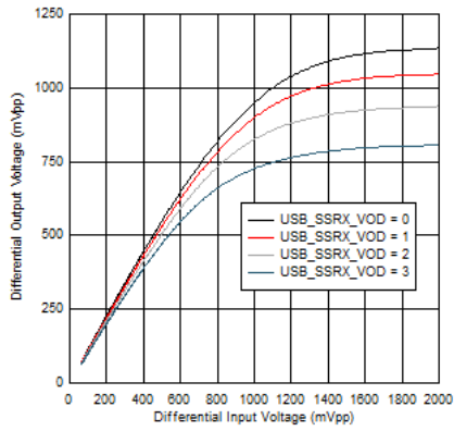
Figure 5-19. USB SSRX VOD Linearity Settings at 5GHz
