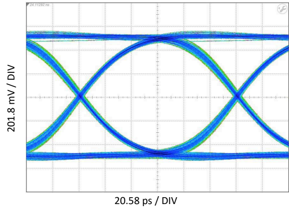
Figure 5-14. DisplayPort HBR3 Eye-Pattern Performance with 12in Input PCB Trace at 8.1Gbps
