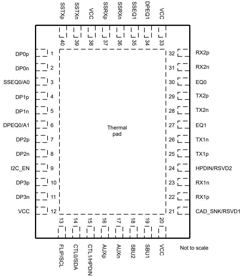
Figure 4-1. TUSB1146-Q1 RGF Package, 40-Pin VQFN (Top View)
