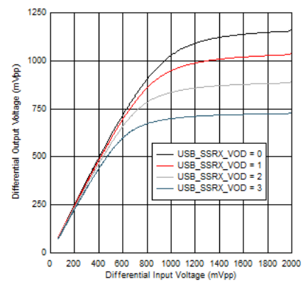
Figure 5-18. USB SSRX VOD Linearity Settings at 100MHz
