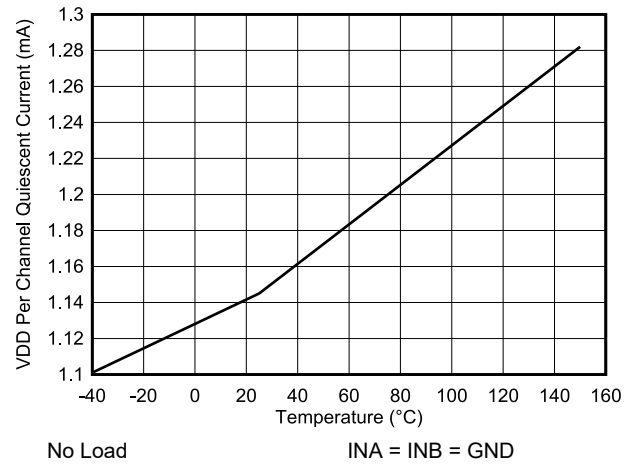
Figure 6-5. VDD Per Channel Quiescent Current ( I_{VDDA} , I_{VDDB} )
