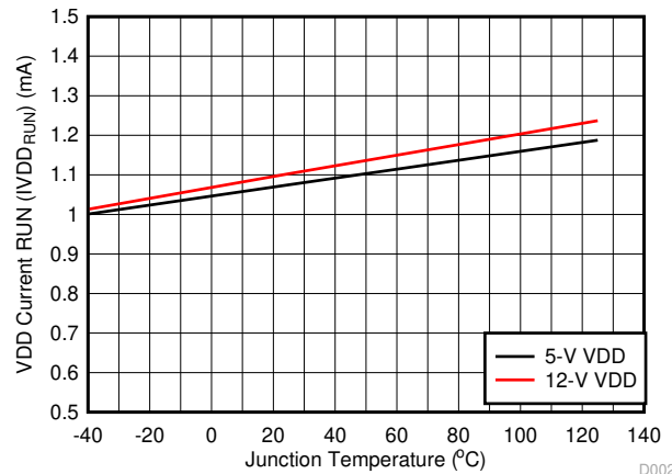
Figure 7-2. Bias Supply Current vs Temperature (No Switching)
