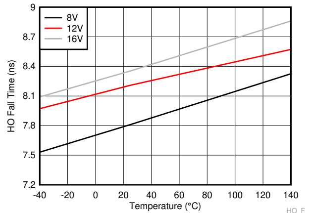
Figure 6-19. HO Fall Time
