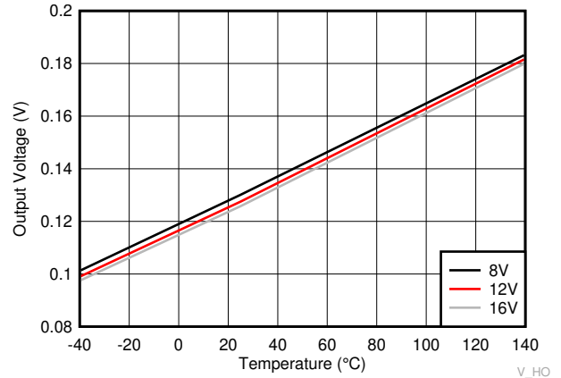
Figure 6-15. HO High Output Voltage ( V_{HOH} )
