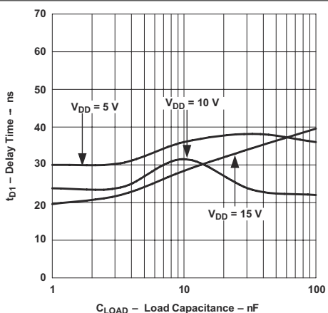
Figure 7-13. t_{D1} Delay Time vs Load Capacitance
