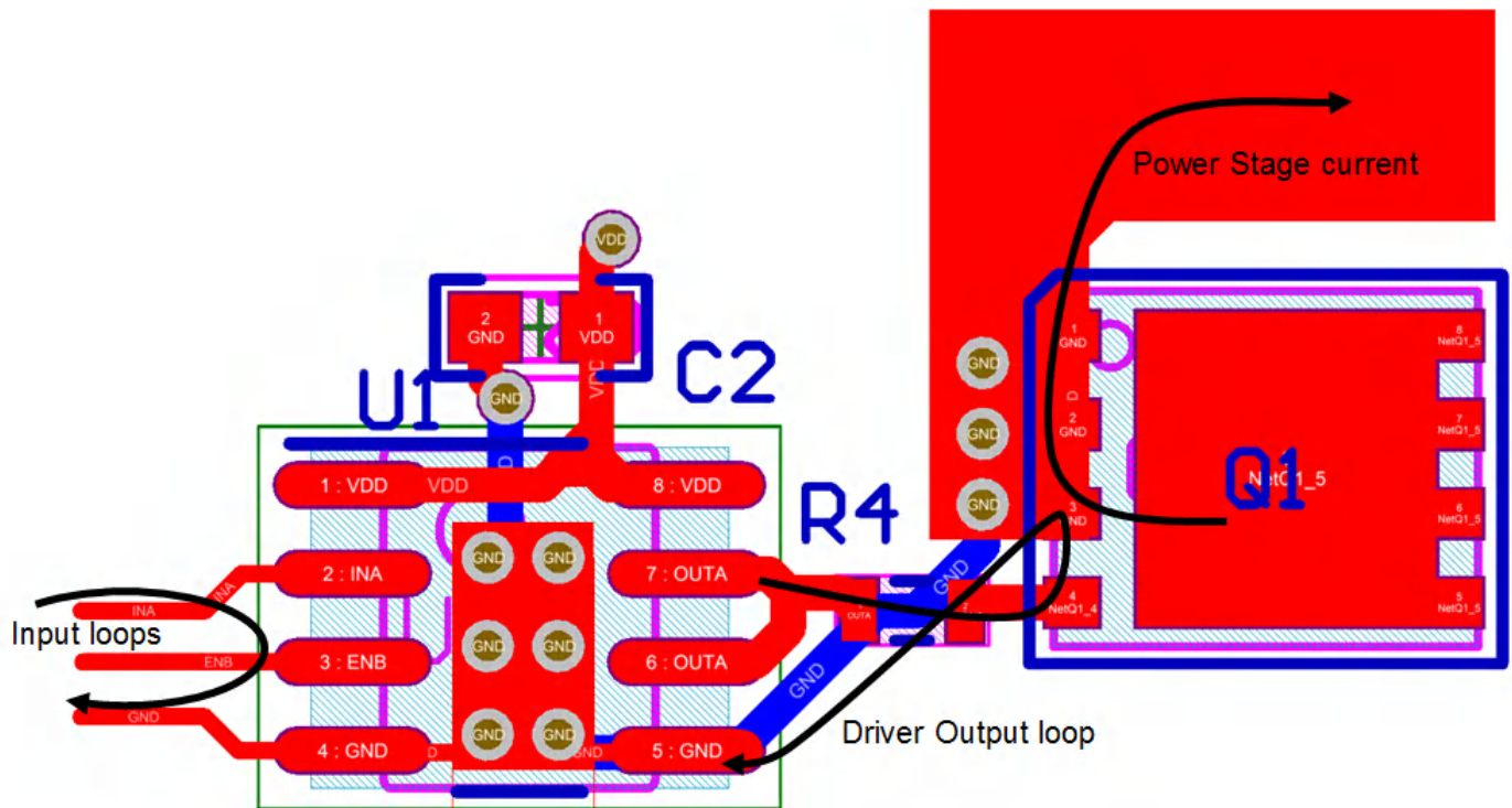
Figure 11-1. Layout Recommendation
