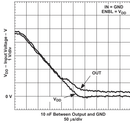
Figure 7-20. Output Behavior vs V_{DD} (UCC27321-Q1)
