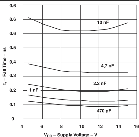
Figure 6-15. Fall Time vs Supply Voltage
