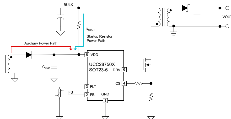
Figure 7-3. Biasing paths in a flyback application
