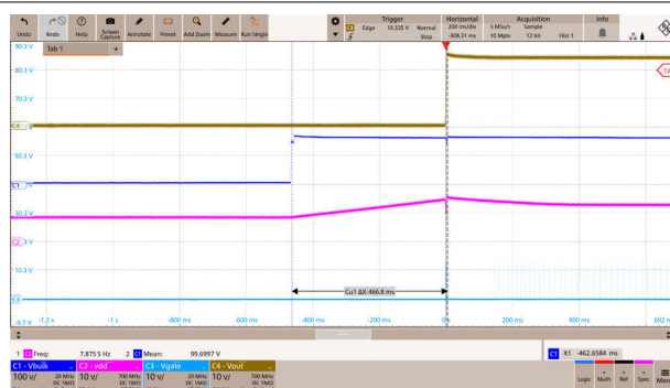
Figure 8-6. Start-Up Waveforms at 115Vac and No Load
