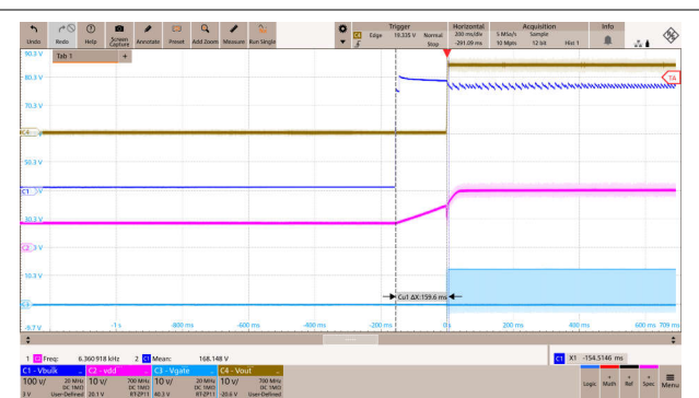
Figure 8-11. Start-Up Waveforms at 265Vac and Full Load
