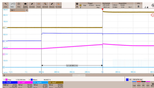
Figure 8-4. Start-Up Waveforms at 85Vac and No Load
