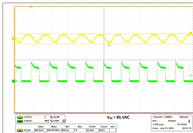
Figure 8-12. Load Transients at 85Vac
