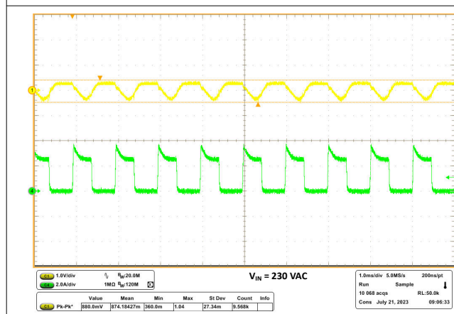
Figure 8-14. Load Transients at 230Vac
