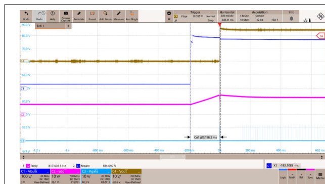
Figure 8-10. Start-Up Waveforms at 265Vac and No Load
