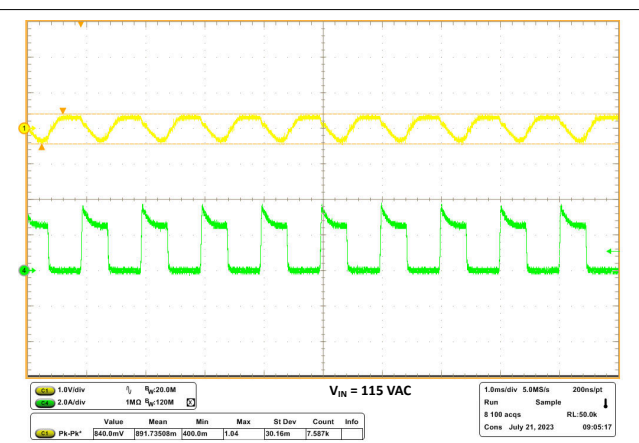
Figure 8-13. Load Transients at 115Vac
