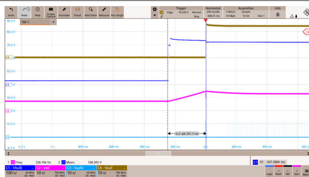
Figure 8-8. Start-Up Waveforms at 230Vac and No Load
