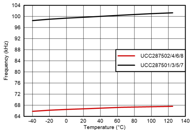
Figure 6-1. Switching Frequency vs Temperature
