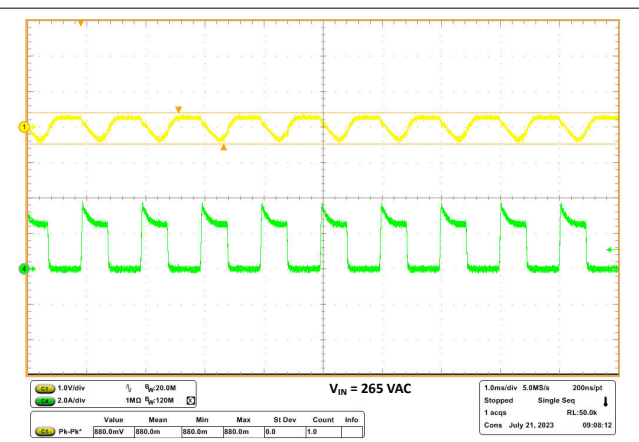
Figure 8-15. Load Transients at 265Vac
