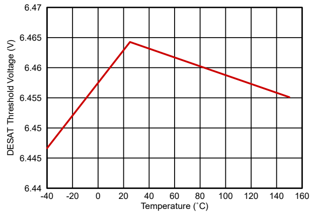
Figure 5-24. DESAT Threshold vs Temperature
