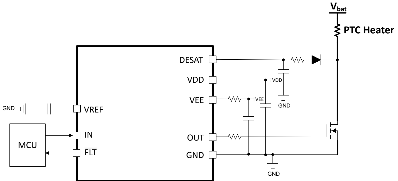
Figure 7-1. UCC57102Z Used in a PTC Heater Application
