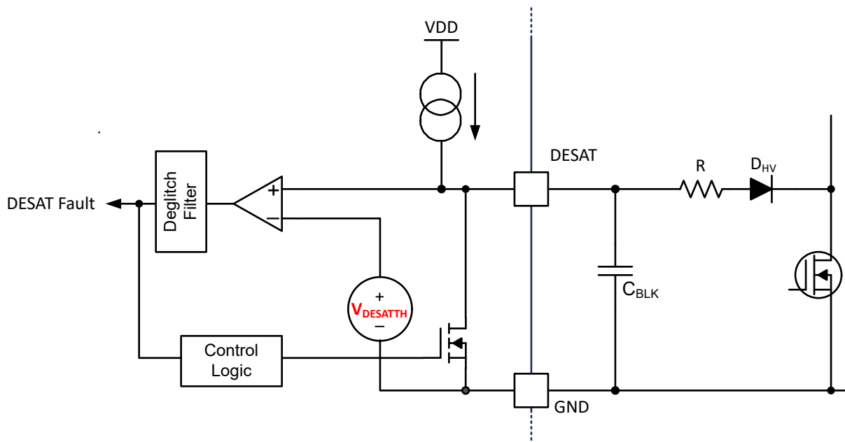
Figure 6-3. DESAT Protection
