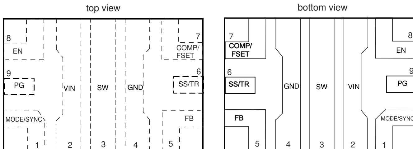
Figure 4-1. Pin Diagram
