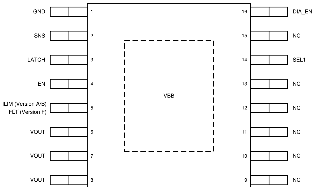
Figure 4-1. Pin Diagram
