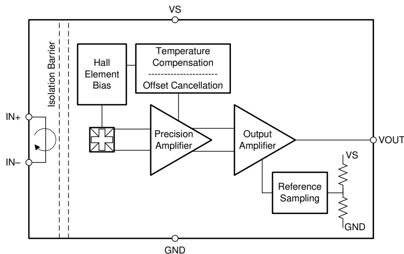
Figure 1-1. TMCS1108-Q1 Functional Block Diagram
