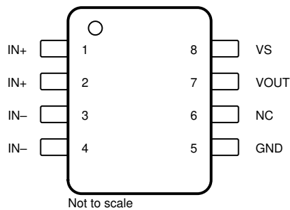
Figure 4-1. TMCS1108-Q1 Pin Diagram
