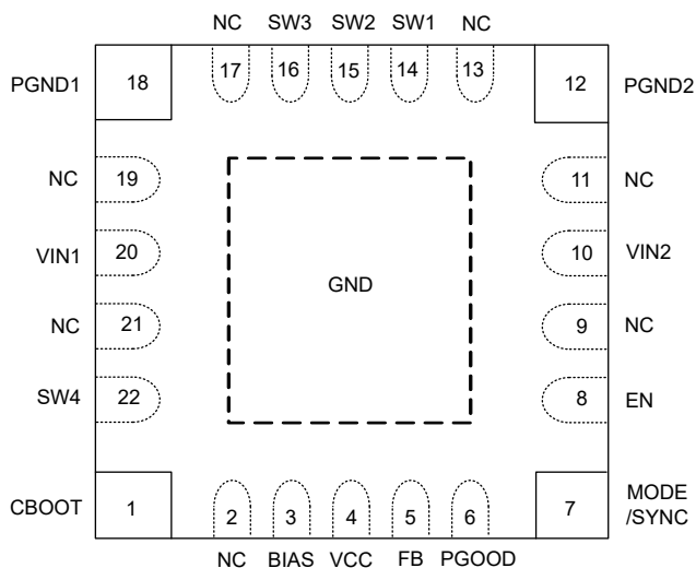
Figure 4-1. Pin Diagram
