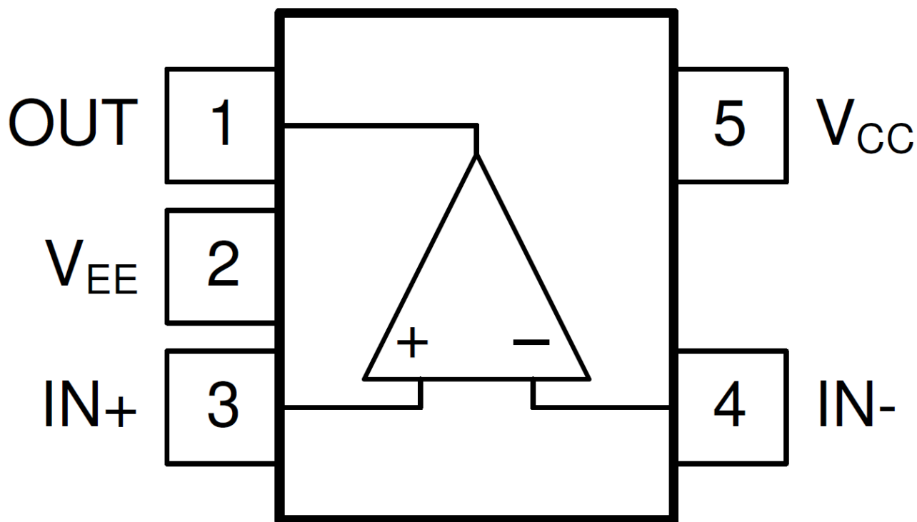
Figure 4-1. Pin Diagram (DCK) Package
