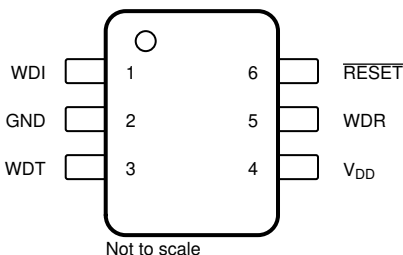
Figure 4-1. Top View 6-Pin SOT-23 DBV Package
