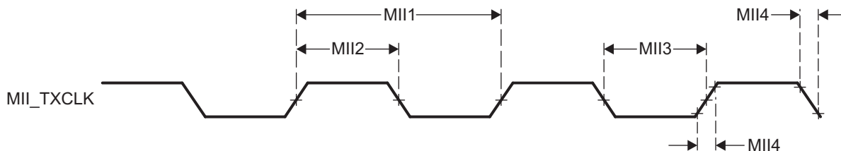
EMAC_MII_02
