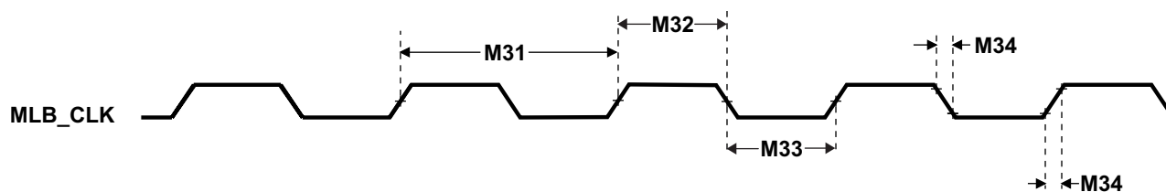
Figure 5-53. MLB_CLK Timing
