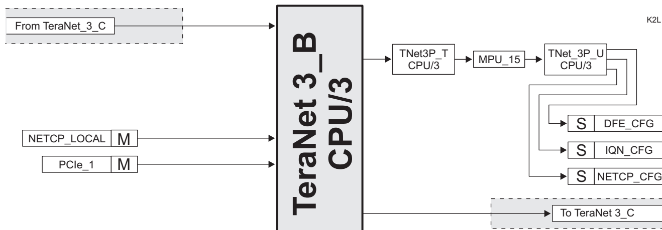
Figure 8-3. TeraNet 3_B
