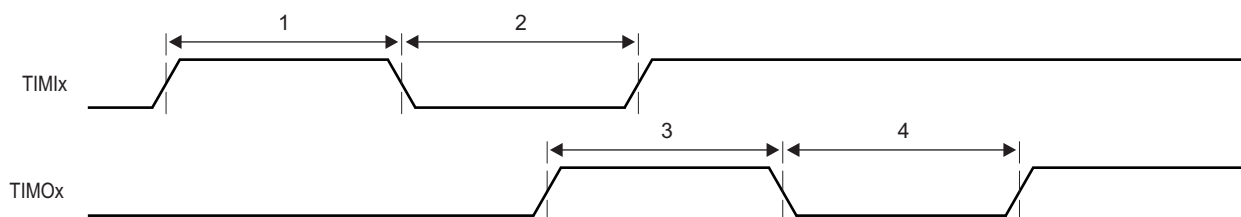
Figure 11-57. Timer Timing
