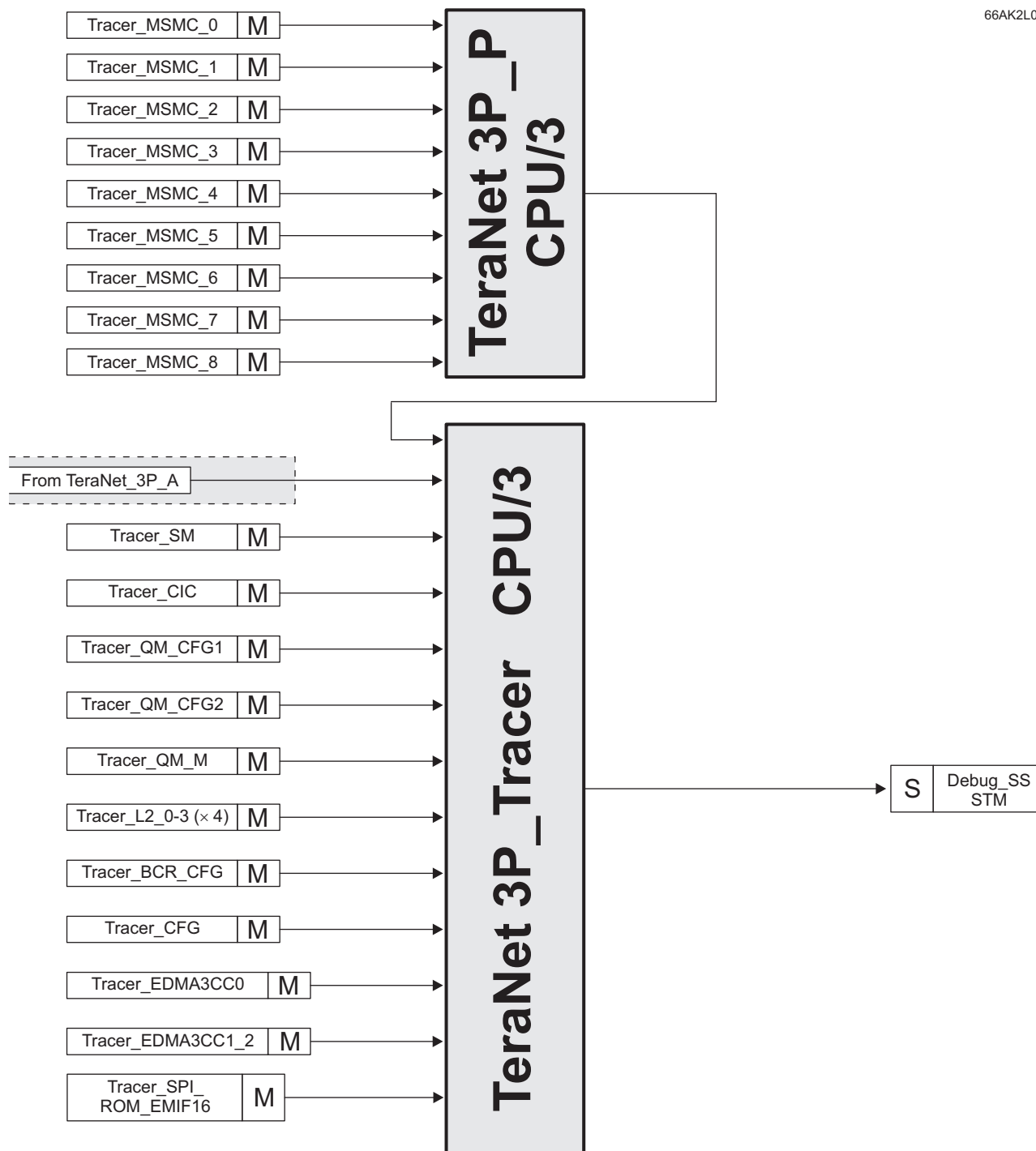
Figure 8-9. TeraNet 3P_Tracer
