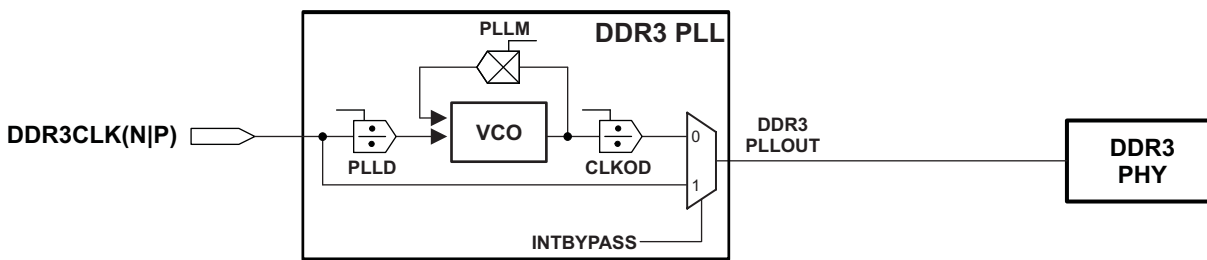
Figure 11-28. DDR3A PLL Block Diagram
