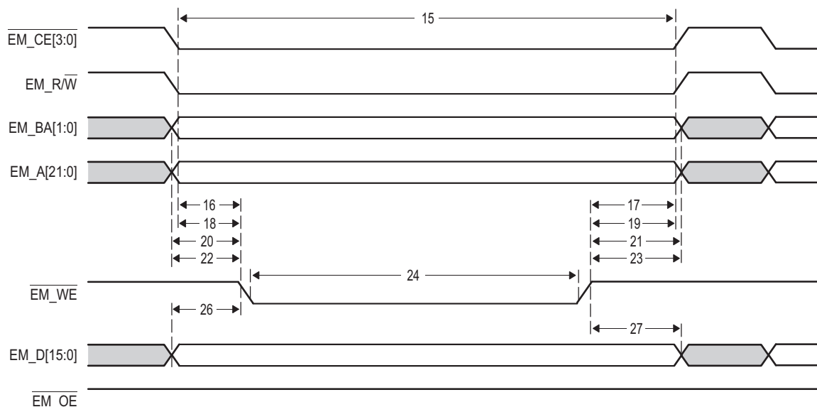
Figure 11-65. EMIF16 Asynchronous Memory Write Timing Diagram
