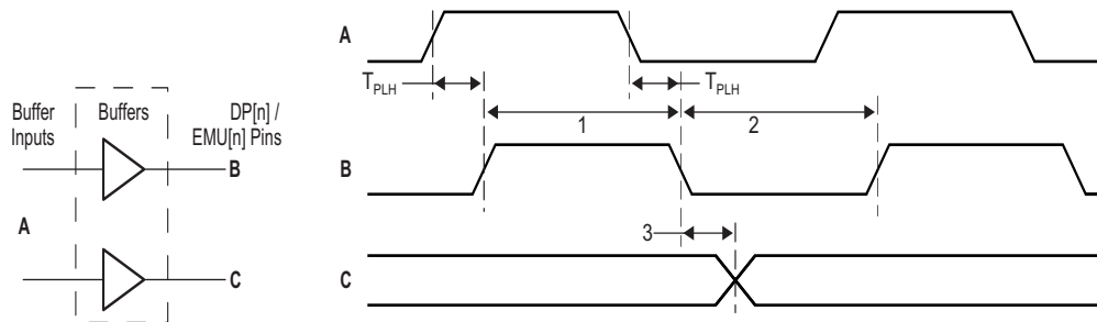
Figure 11-68. Trace Timing
