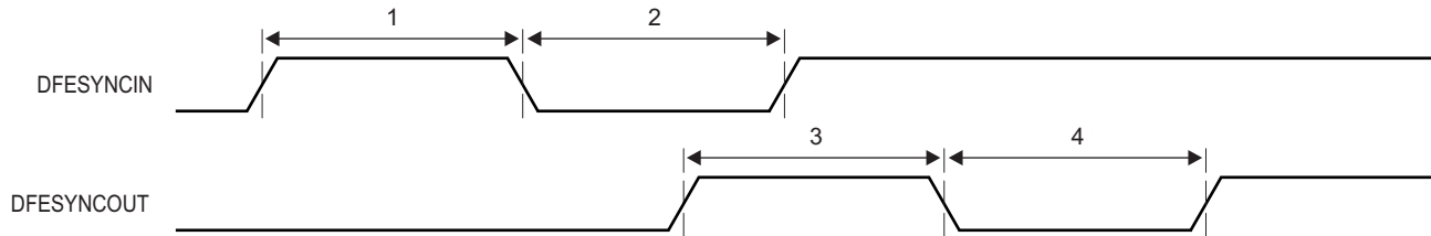
Figure 11-40. DFESYN CIN Sync Input Pulse Timing
