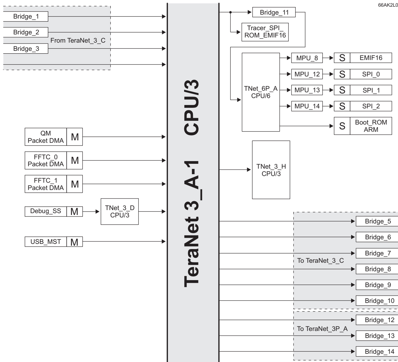
Figure 8-1. TeraNet 3_A-1
