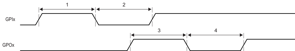
Figure 11-58. GPIO Timing
