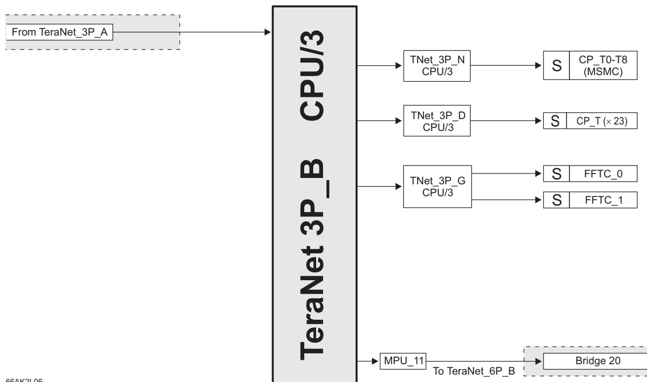
Figure 8-7. TeraNet 3P_B
