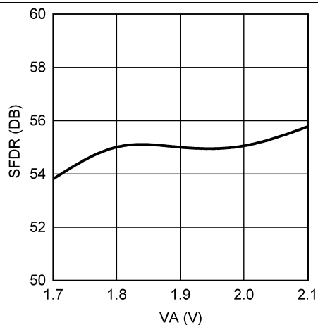
Figure 31. SFDR vs. SUPPLY VOLTAGE
