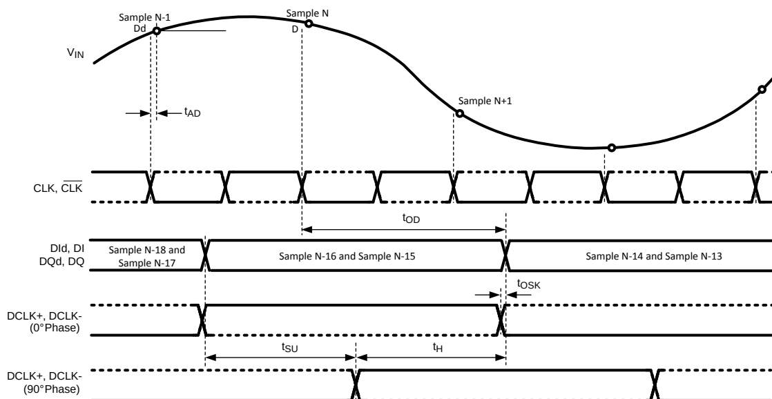
Figure 4. ADC08D502 Timing — DDR Clocking
