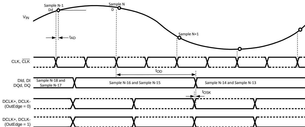
Figure 3. ADC08D502 Timing — SDR Clocking
