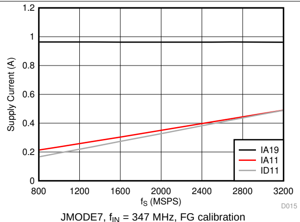
Figure 45. Supply Current vs Sampling Rate
