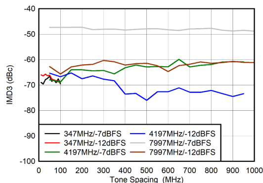
Figure 5-102. DES Mode: IMD3 vs Tone Spacing
