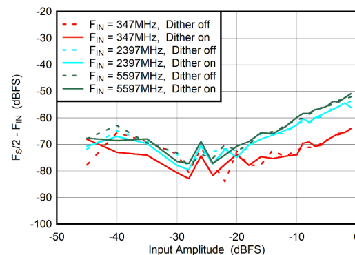
Figure 5-66. DES Mode: F_S/2 - F_{\text{IN}} vs Input Amplitude and Dither
