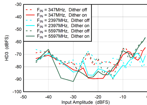
Figure 5-64. DES Mode: HD3 vs Input Amplitude and Dither
