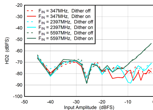
Figure 5-62. DES Mode: HD2 vs Input Amplitude and Dither
