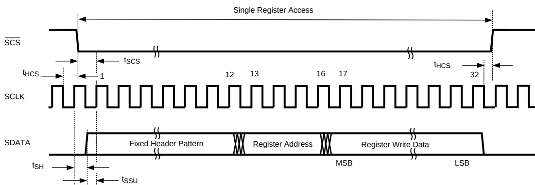
Figure 5. Serial Interface Timing
