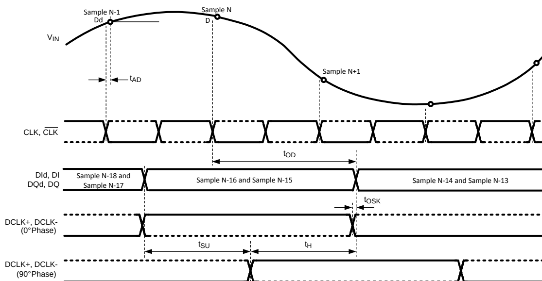
Figure 3. ADC08DL500 Timing — DDR Clcking in 1:2 Demultiplexed Mode
