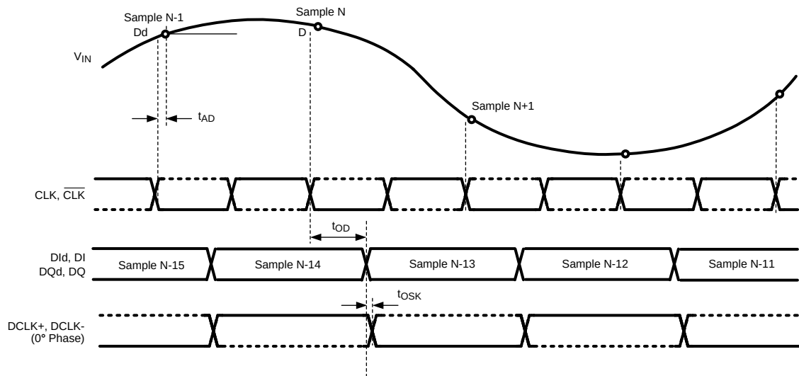
Figure 4. ADC08DL500 Timing — DDR Clocking in Non-Demultiplexed Mode
