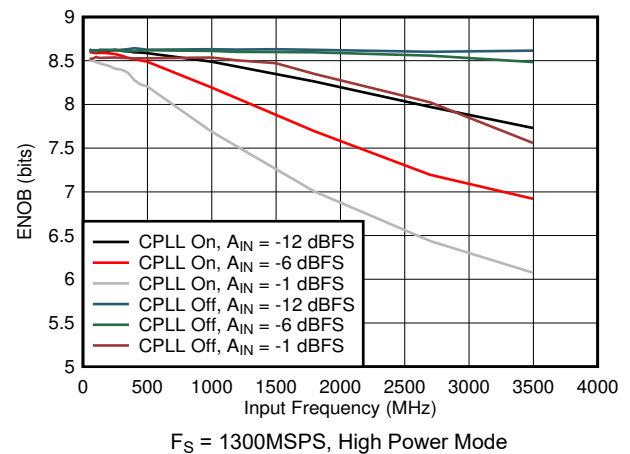
Figure 5-72. ENOB vs Input Frequency, CPLL and Input Amplitude
