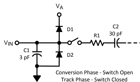
Figure 38. Equivalent Input Circuit
