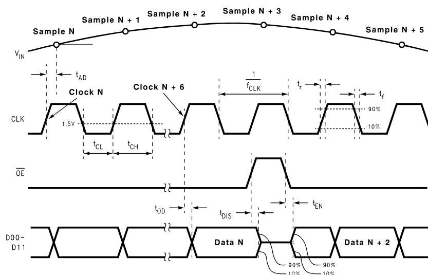
Figure 1. Output Timing
