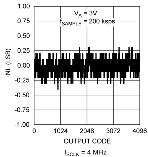
Figure 5. INL
