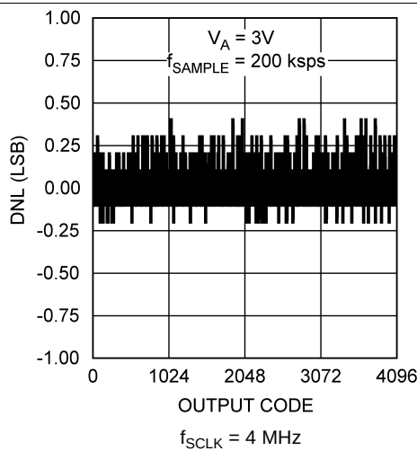
Figure 4. DNL
