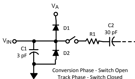
Figure 50. Equivalent Input Circuit
