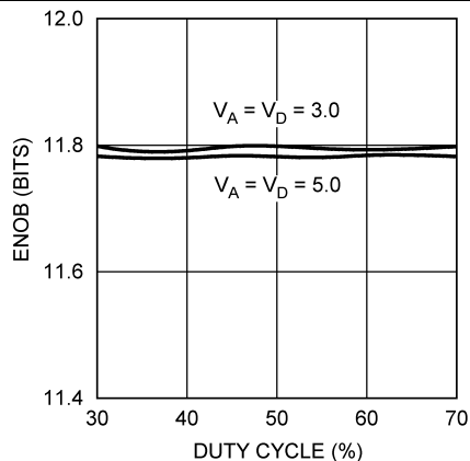
Figure 19. ENOB vs SCLK Duty Cycle
