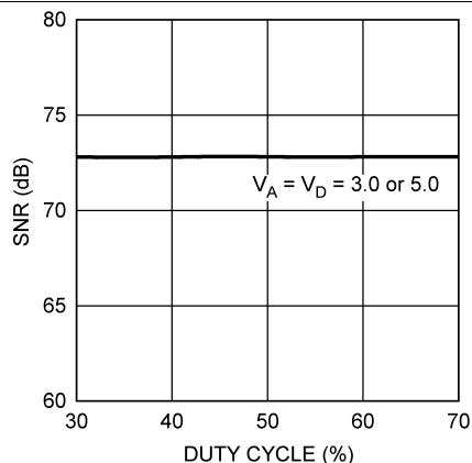
Figure 17. SNR vs SCLK Duty Cycle
