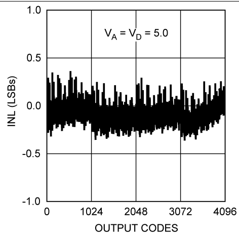
Figure 7. INL
