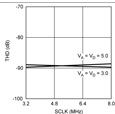
Figure 23. THD vs SCLK
