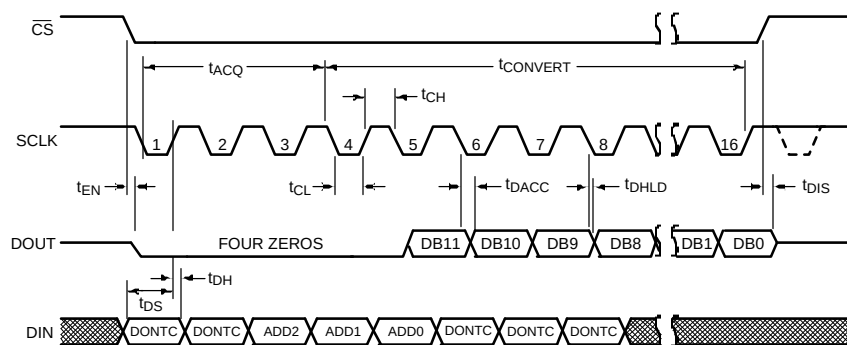
Figure 2. ADC128S052 Serial Timing Diagram
