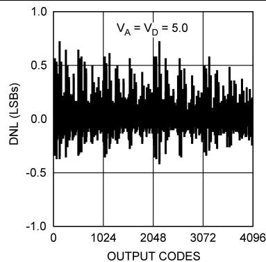
Figure 5. DNL
