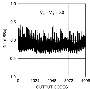
Figure 7. INL
