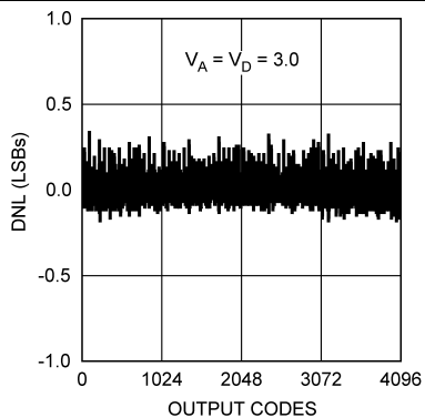
Figure 4. DNL
