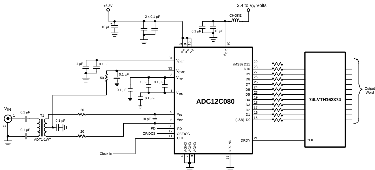
Figure 34. Application Circuit
