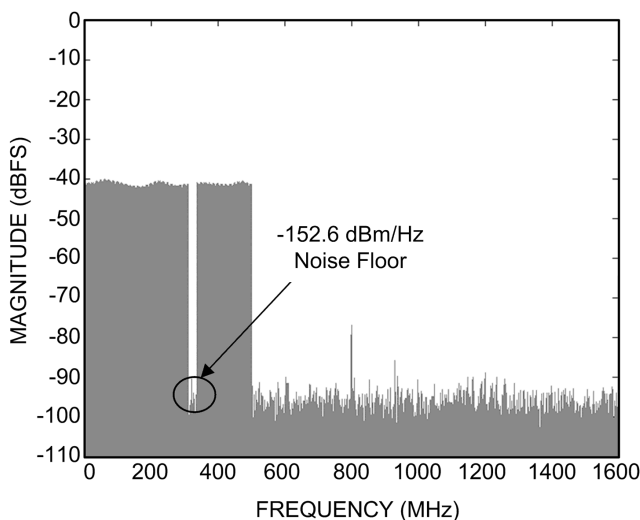
Wideband Performance
