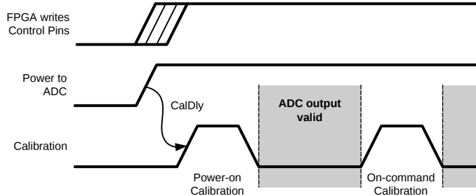
Figure 76. Power-On With Control Pins Set by FPGA Pre Power-on Cal
