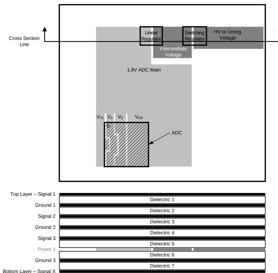
Figure 6-10. Power and Grounding Example
