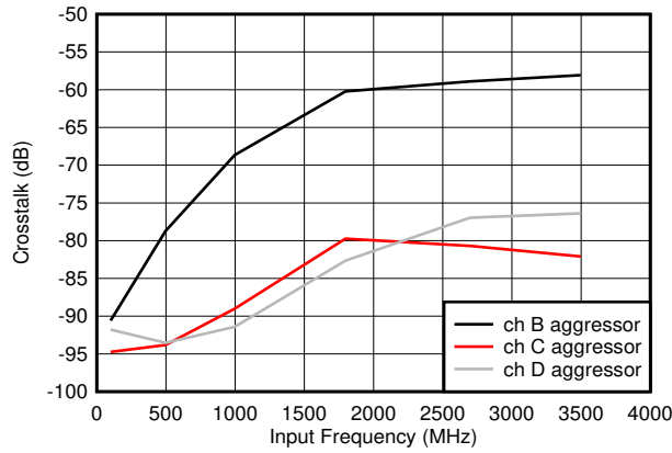
Figure 6-77. Crosstalk to Channel A vs F_{IN}
