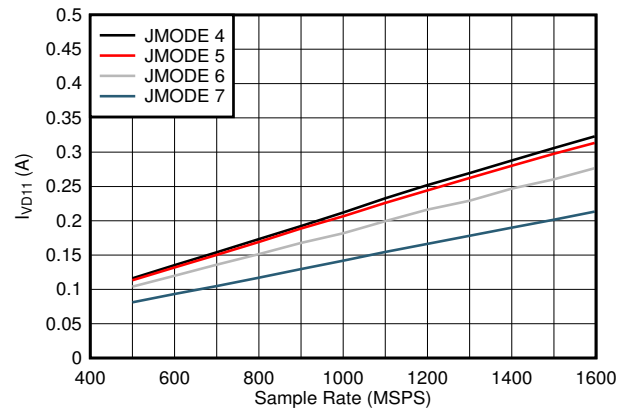
Figure 6-106. Single Channel, I_{VD11} vs F_S and JMODE 4 - 7
