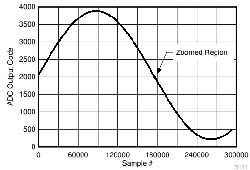
Figure 6-126. Background Calibration Core Transition (AC Signal)
