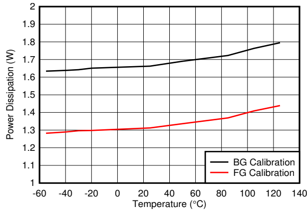
Figure 6-123. Single Channel, Power Dissipation vs Temperature
