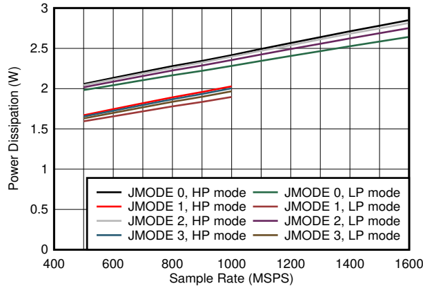
Low power background calibration mode Figure 6-79. Quad Channel, Power Dissipation vs F_S and JMODES 0 - 3
