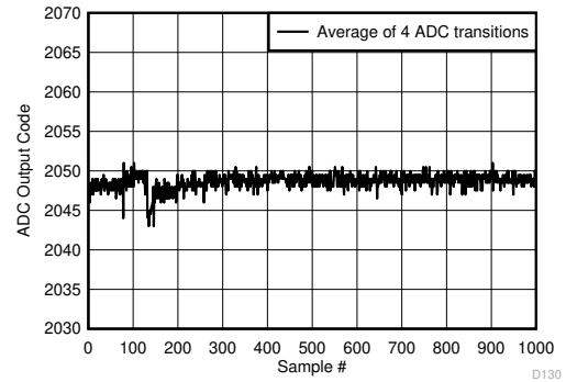
Figure 6-124. Background Calibration Core Transition (midscale voltage)
