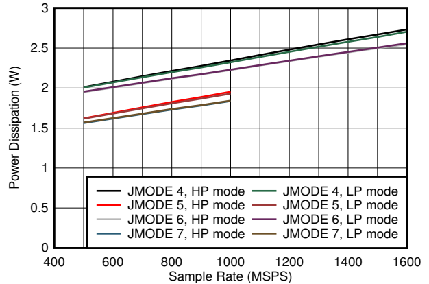
Low power background calibration mode Figure 6-80. Quad Channel, Power Dissipation vs F_S and JMODE 4 - 7
