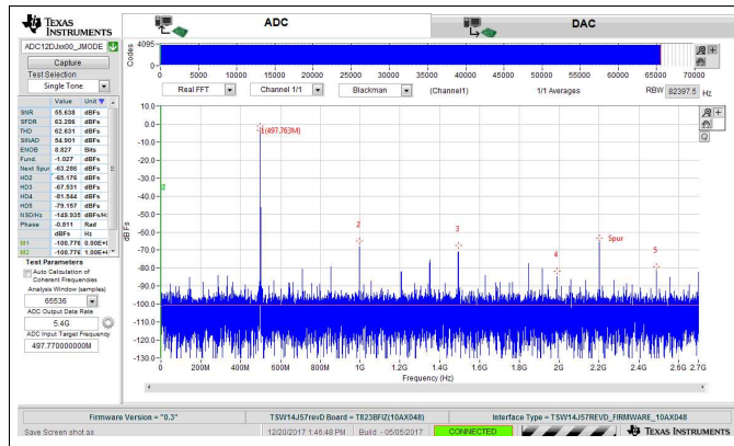
Figure 181. FFT for 497.77-MHz Input Signal, 5.4 GSPS, JMODE0
