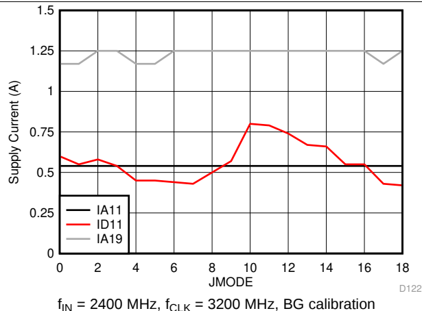
Figure 58. Supply Current vs JMODE
