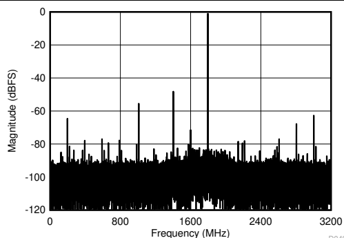
JMODE 1, FG calibration, f_s = 6400\text{MSPS} , SNR = 51.4dBFS, SFDR = 48dBFS, ENOB = 7.3 bits
