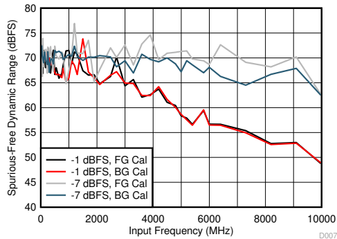
JMODE 3, f_s = 3200\text{MHz} , FG and BG calibration
