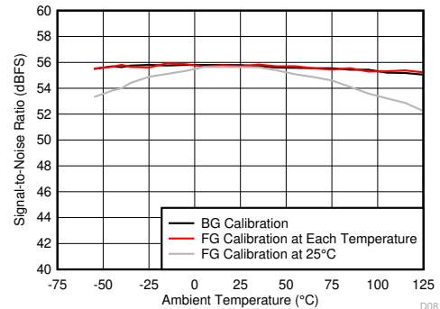
Figure 5-51. SNR vs Temperature and Calibration Mode
