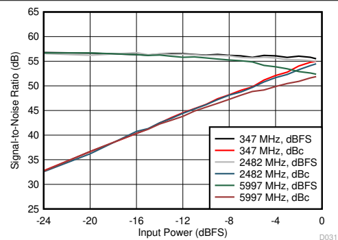
JMODE 1, FG calibration, f_s = 6400\text{MSPS}
