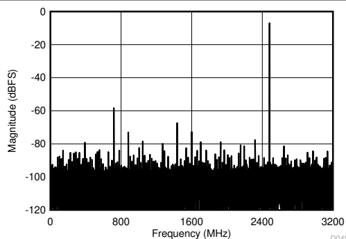
JMODE 1, FG calibration, f_s = 6400\text{MSPS} , SNR = 56.1dBFS, SFDR = 58dBFS, ENOB = 8.6 bits
