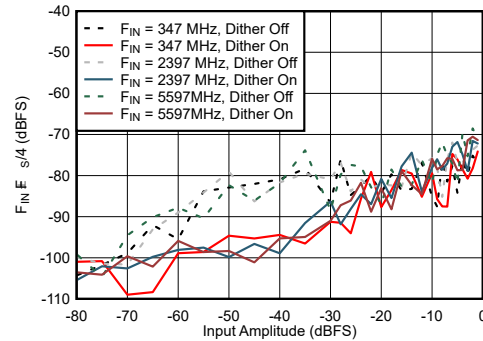
Figure 6-66. DES Mode: F_{\text{IN}} \pm F_{\text{IN}}/4 vs Input Amplitude and Dither
