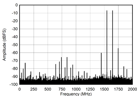
Figure 6-25. Dual Channel Mode: Two Tone FFT at 2397 MHz
