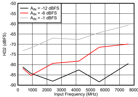
Figure 6-79. DES Mode: HD2 vs Input Frequency
