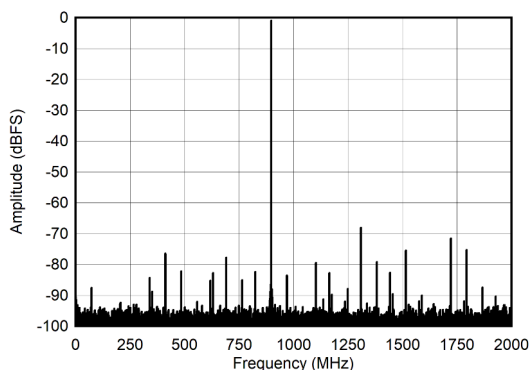
Figure 6-19. Dual Channel Mode: Single Tone FFT at 897 MHz
