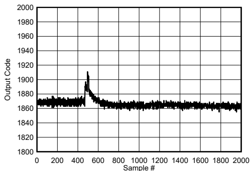
Figure 6-138. Background Calibration Core Transition (DC Offset Signal)
