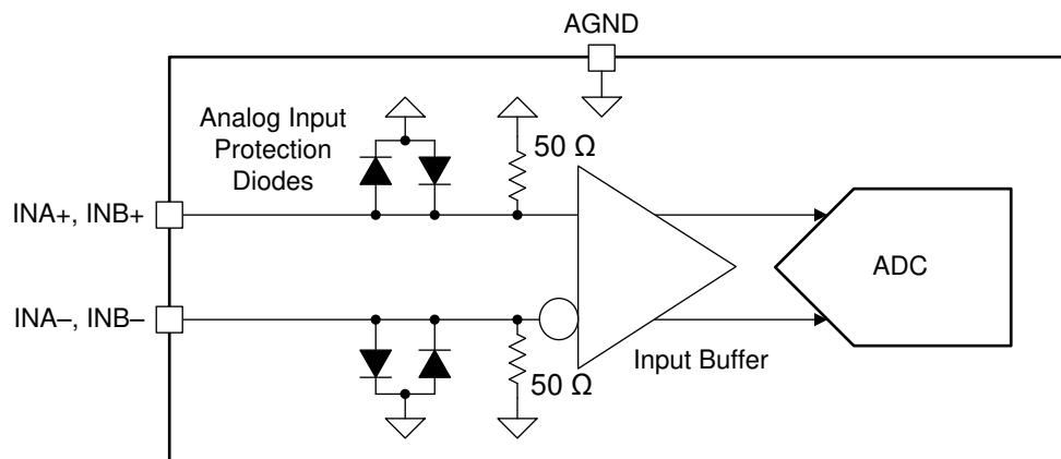
Figure 7-1. ADC12DJ4000RF Analog Input Internal Termination and Protection Diagram
