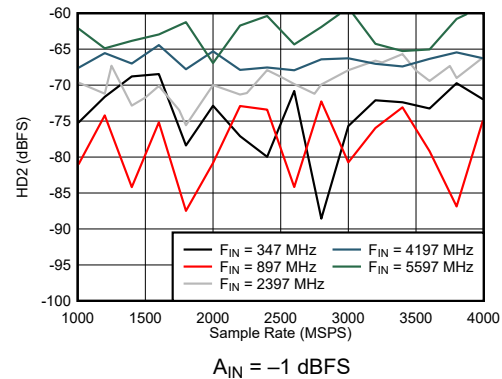
Figure 6-48. Dual Channel Mode: HD2 vs Sample Rate and Input Frequency
