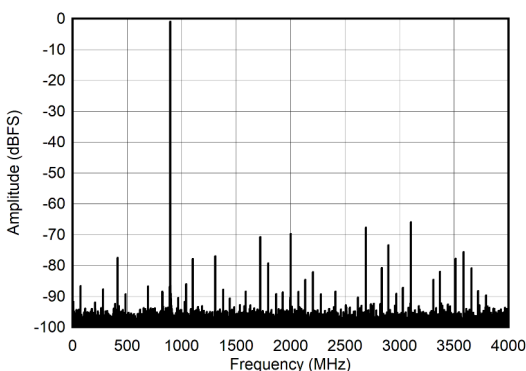
Figure 6-9. DES Mode: Single Tone FFT at 897 MHz
