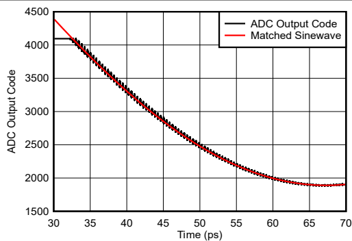
Figure 6-144. Sinewave Overdrive Recovery
