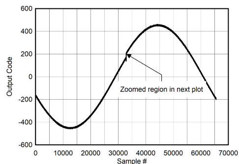
Figure 6-139. Background Calibration Core Transition (AC Signal)
