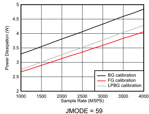
Figure 6-135. Dual Channel Mode: Power Dissipation vs Sample Rate
