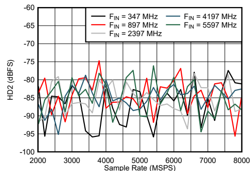
Figure 6-36. DES Mode: HD2 vs Sample Rate and Input Frequency
