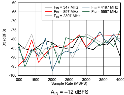
Figure 6-53. Dual Channel Mode: HD3 vs Sample Rate and Input Frequency
