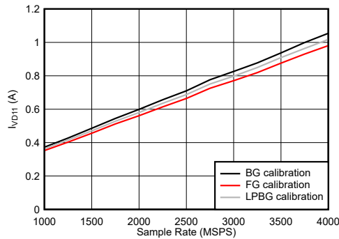
Figure 6-120. DES Mode: I_{VD11} vs Sample Rate
