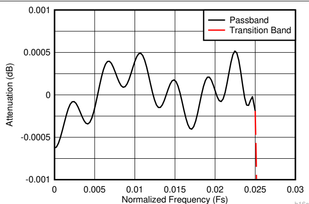
Figure 7-16. Decimate-by-16 Composite Zoomed Pass-Band Response
