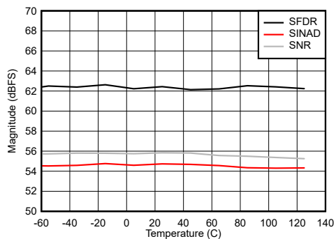
Figure 6-92. DES Mode: SNR, SINAD and SFDR vs Temperature
