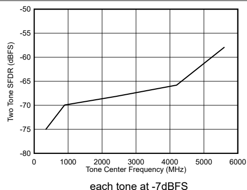
Figure 6-110. DES Mode: Two Tone SFDR vs Input Frequency
