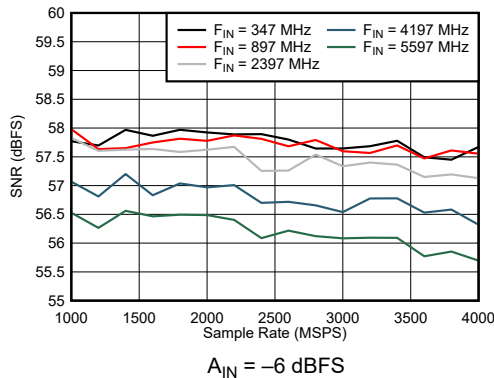
Figure 6-43. Dual Channel Mode: SNR vs Sample Rate and Input Frequency
