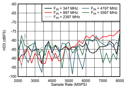
Figure 6-37. DES Mode: HD3 vs Sample Rate and Input Frequency
