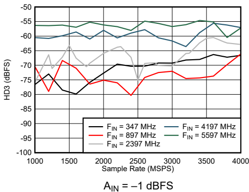
Figure 6-51. Dual Channel Mode: HD3 vs Sample Rate and Input Frequency
