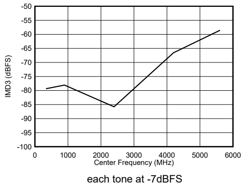
Figure 6-105. Dual Channel Mode: IMD3 vs Input Frequency
