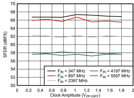
Figure 6-89. DES Mode: SFDR vs Clock Amplitude
