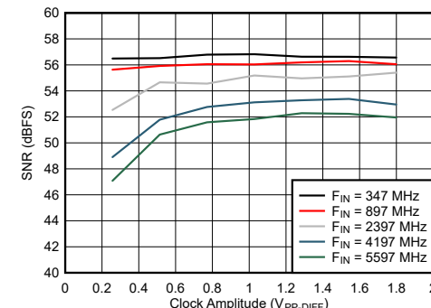
Figure 6-88. DES Mode: SNR vs Clock Amplitude
