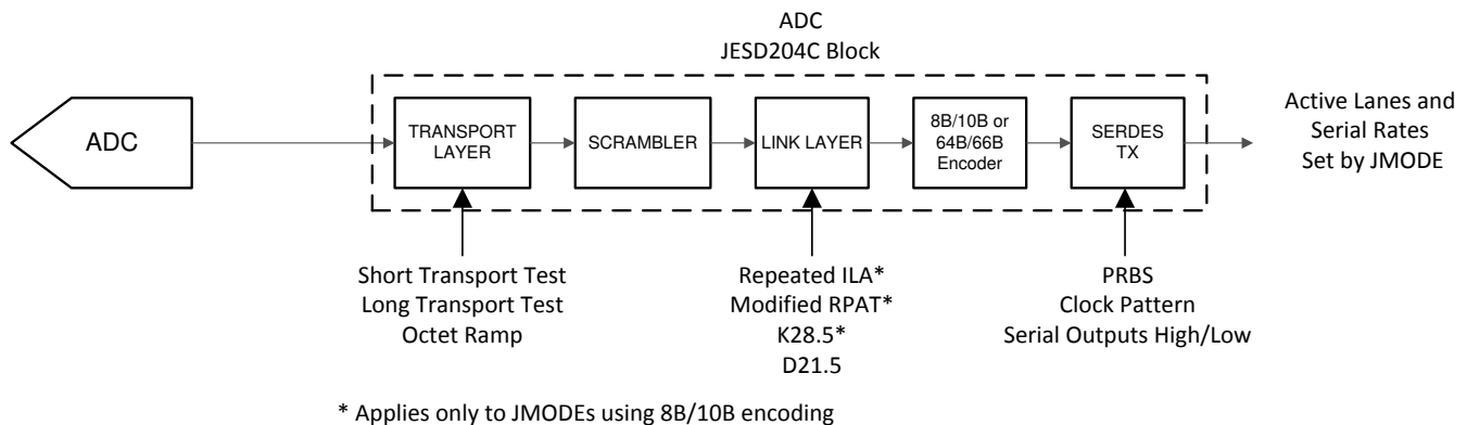
Figure 7-25. Test Mode Insertion Points
