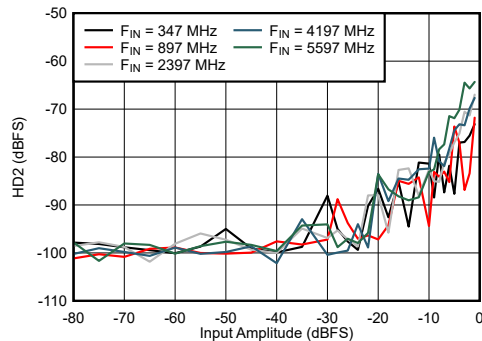
Figure 6-59. DES Mode: HD2 vs Input Amplitude and Frequency
