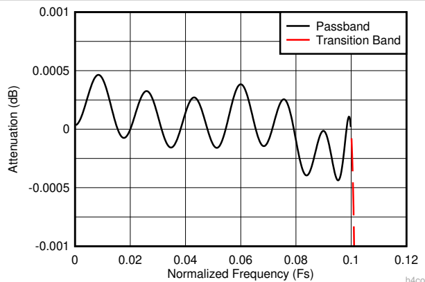
Figure 7-12. Decimate-by-4 Composite Zoomed Pass-Band Response
