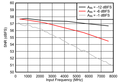
Figure 6-82. DES Mode: F_{\text{IN}} \pm F_S/4 vs Input Frequency
