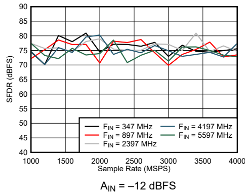
Figure 6-47. Dual Channel Mode: SFDR vs Sample Rate and Input Frequency
