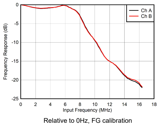
Figure 6-3. Dual Channel Mode: Input Amplitude vs Input Frequency
