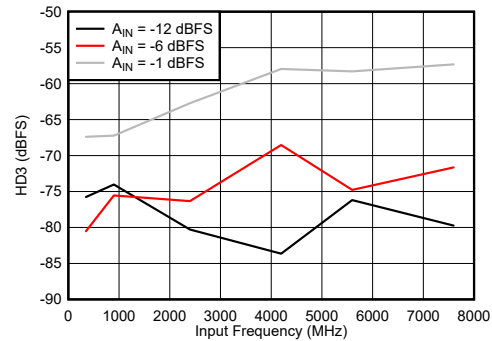
Figure 6-80. DES Mode: HD3 vs Input Frequency
