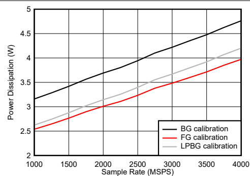
Figure 6-123. DES Mode: Power Dissipation vs Sample Rate
