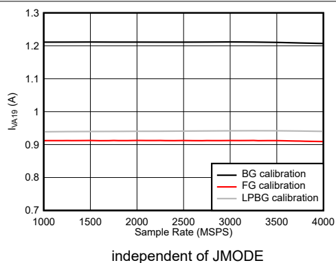
Figure 6-116. DES Mode: I_{VA19} vs Sample Rate
