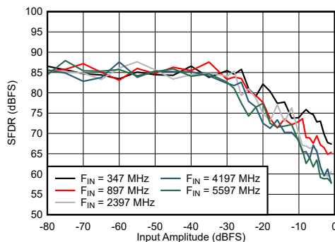
Figure 6-57. DES Mode: SFDR vs Input Amplitude and Frequency
