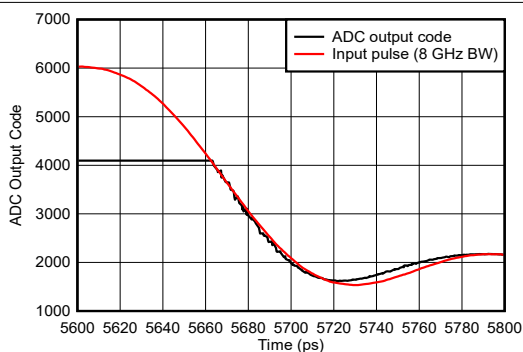
Figure 6-142. Pulse Overdrive Recovery Zoomed
