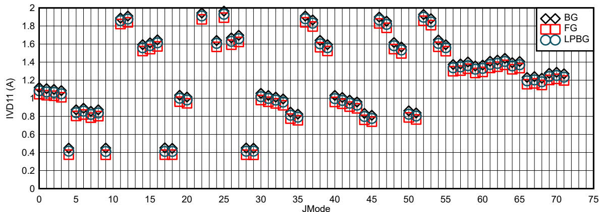
Figure 6-115. I_{VD11} vs \text{JMODE} at F_{\text{CLK}} = 4\text{ GHz}
