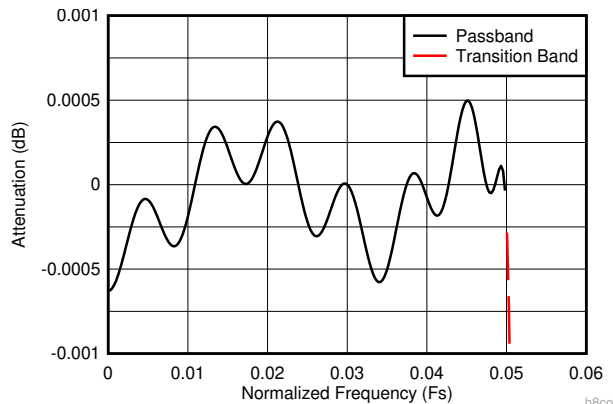
Figure 7-14. Decimate-by-8 Composite Zoomed Pass-Band Response
