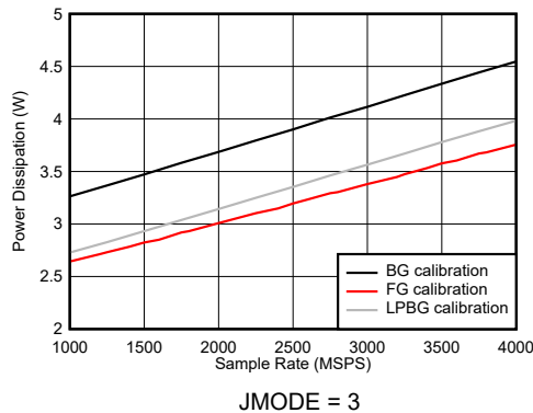
Figure 6-132. Dual Channel Mode: Power Dissipation vs Sample Rate
