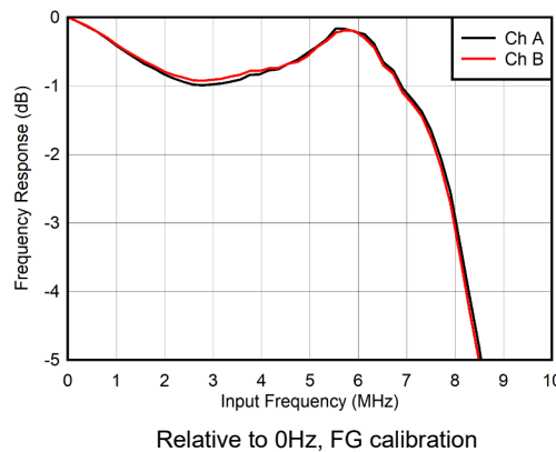
Figure 6-4. Input Response vs Input Frequency (zoomed)
