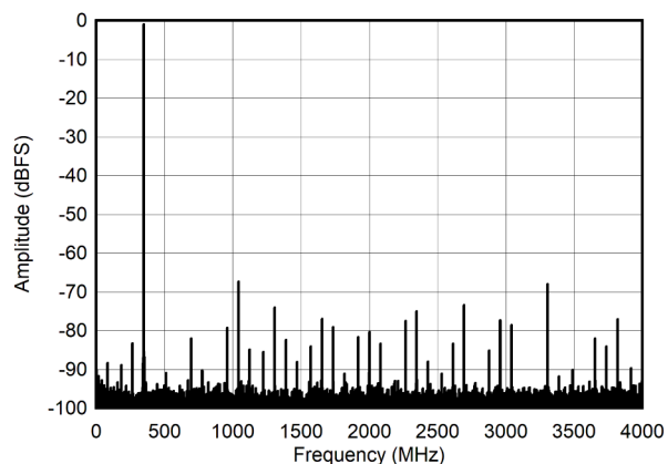
Figure 8-2. FFT for 347 MHz Input Signal, 8 GSPS, JMODE1
