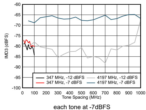
Figure 6-108. DES Mode: IMD3 vs Tone Spacing
