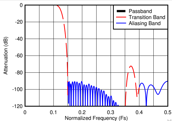
Figure 7-11. Decimate-by-4 Composite Response
