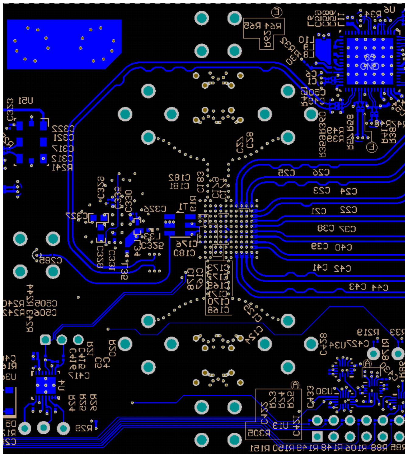
Figure 8-8. Bottom Layer Routing: Additional CLK Routing, DA4-7, DB4-7
