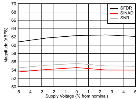
Figure 6-100. DES Mode: SNR, SINAD and SFDR vs Supply Voltage
