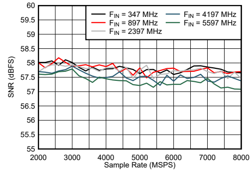
Figure 6-30. DES Mode: SNR vs Sample Rate and Input Frequency
