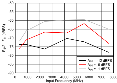
Figure 6-81. DES Mode: F_S/2 - F_{\text{IN}} vs Input Frequency
