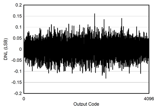
Figure 6-6. DNL vs ADC Code
