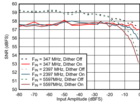
Figure 6-68. Dual Channel Mode: SNR vs Input Amplitude and Dither
