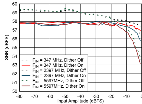
Figure 6-56. DES Mode: SNR vs Input Amplitude and Dither
