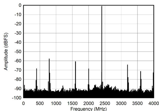
Figure 6-12. DES Mode: Single Tone FFT at 5597 MHz
