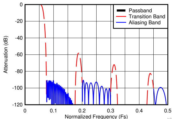
Figure 7-13. Decimate-by-8 Composite Response
