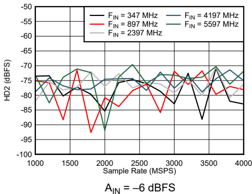
Figure 6-49. Dual Channel Mode: HD2 vs Sample Rate and Input Frequency
