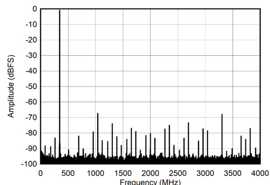
Figure 6-8. DES Mode: Single Tone FFT at 347 MHz
