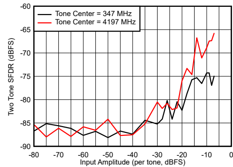
Figure 6-112. DES Mode: Two Tone SFDR vs Input Amplitude
