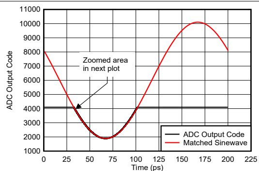
Figure 6-143. Sinewave Overdrive Recovery
