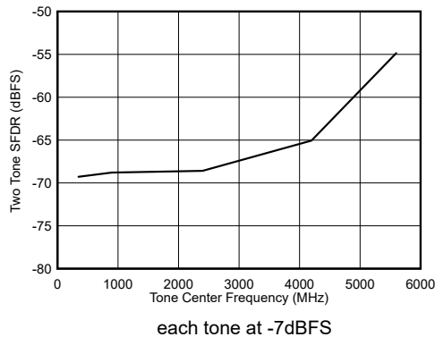
Figure 6-111. Dual Channel Mode: Two Tone SFDR vs Input Frequency
