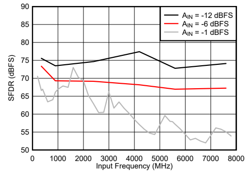
Figure 6-84. Dual Channel Mode: SFDR vs Input Frequency
