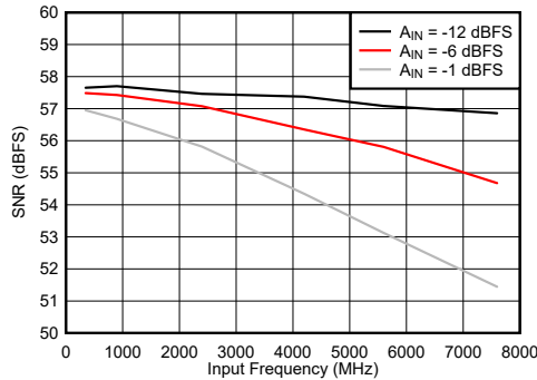
Figure 6-77. DES Mode: SNR vs Input Frequency
