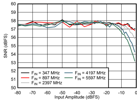
Figure 6-67. Dual Channel Mode: SNR vs Input Amplitude and Frequency
