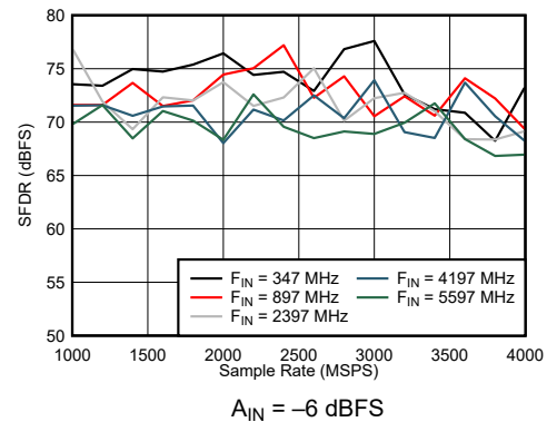
Figure 6-46. Dual Channel Mode: SFDR vs Sample Rate and Input Frequency
