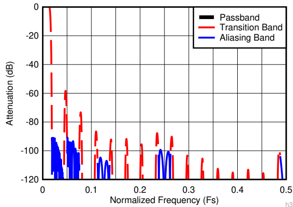
Figure 7-17. Decimate-by-32 Composite Response
