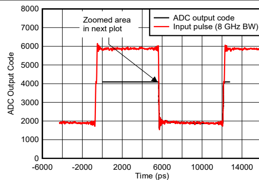
Figure 6-141. Pulse Overdrive Recovery
