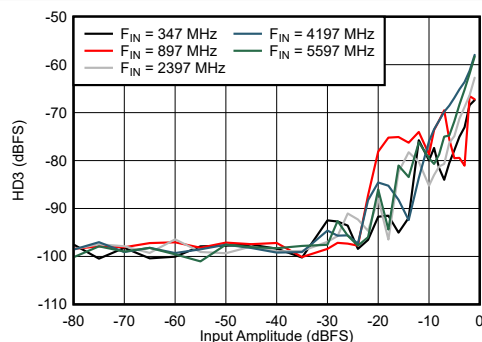
Figure 6-61. DES Mode: HD3 vs Input Amplitude and Frequency
