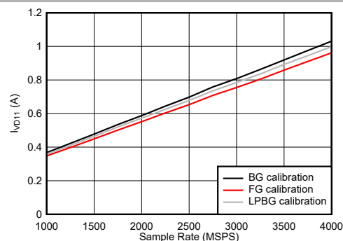
Figure 6-128. Dual Channel Mode: I_{VD11} vs Sample Rate
