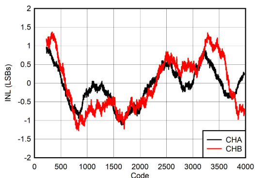
Figure 6-7. INL vs ADC Code
