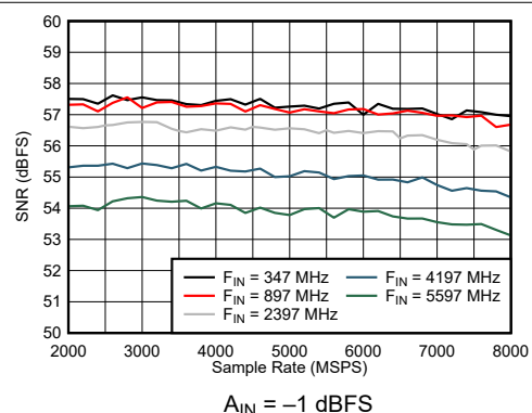
Figure 6-28. DES Mode: SNR vs Sample Rate and Input Frequency
