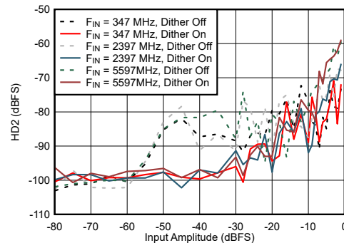
Figure 6-72. Dual Channel Mode: HD2 vs Input Amplitude and Dither
