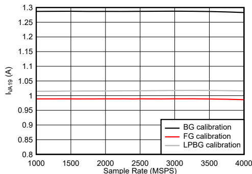
Figure 6-126. Dual Channel Mode: I_{VA19} vs Sample Rate
