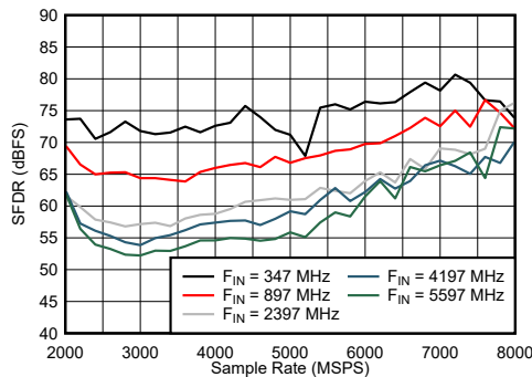
Figure 6-31. DES Mode: SFDR vs Sample Rate and Input Frequency
