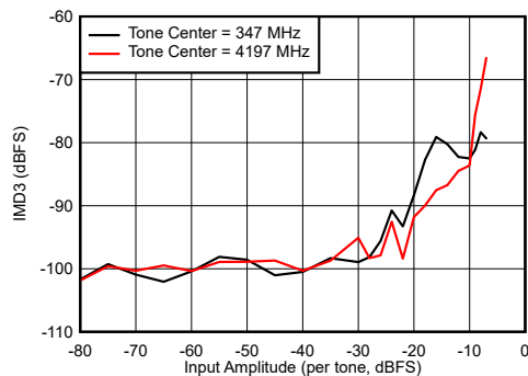
Figure 6-107. Dual Channel Mode: IMD3 vs Input Amplitude
