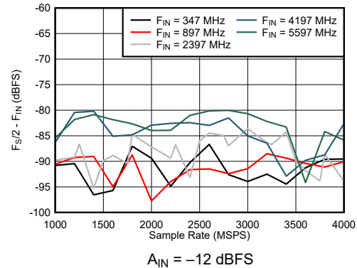
Figure 6-54. Dual Channel Mode: F_{\text{S}}/2 - F_{\text{IN}} vs Sample Rate and Input Frequency
