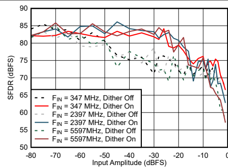
Figure 6-70. Dual Channel Mode: SFDR vs Input Amplitude and Dither
