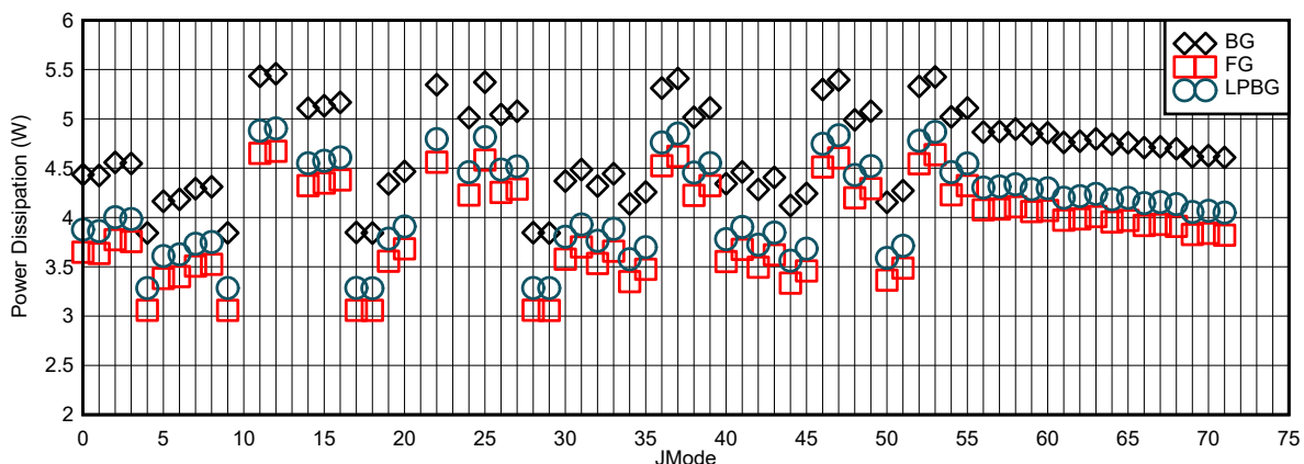
Figure 6-114. Power Dissipation vs JMODE at F_{\text{CLK}} = 4\text{ GHz}
