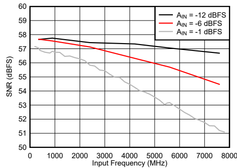
Figure 6-83. Dual Channel Mode: SNR vs Input Frequency
