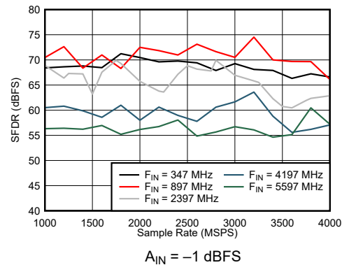
Figure 6-45. Dual Channel Mode: SFDR vs Sample Rate and Input Frequency
