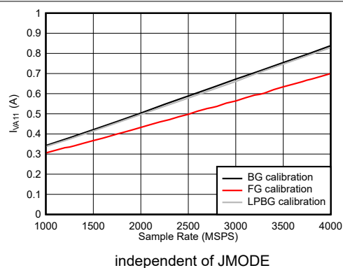
Figure 6-117. DES Mode: I_{VA11} vs Sample Rate
