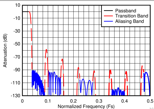
Figure 7-15. Decimate-by-16 Composite Response
