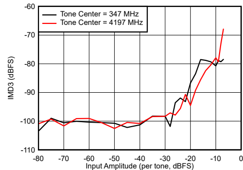
Figure 6-106. DES Mode: IMD3 vs Input Amplitude
