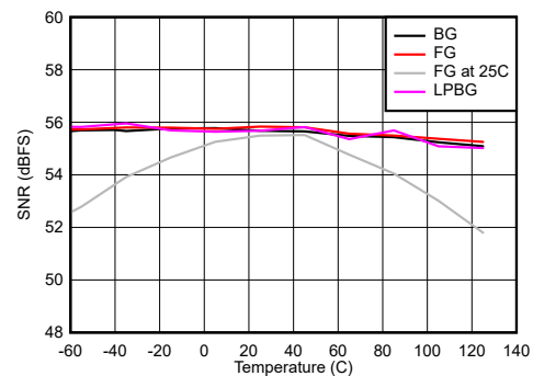
Figure 6-96. DES Mode: SNR vs Temperature and Calibration Mode
