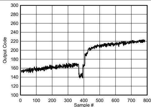
Figure 6-140. Background Calibration Core Transition (AC Signal Zoomed)
