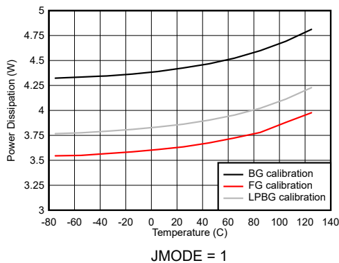
Figure 6-136. DES Mode: Power Dissipation vs Temperature
