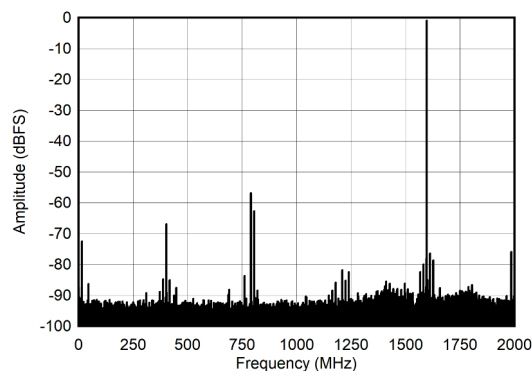
Figure 6-22. Dual Channel Mode: Single Tone FFT at 5597 MHz
