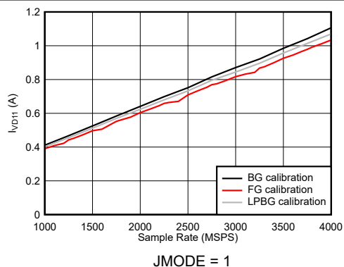
Figure 6-118. DES Mode: I_{VD11} vs Sample Rate
