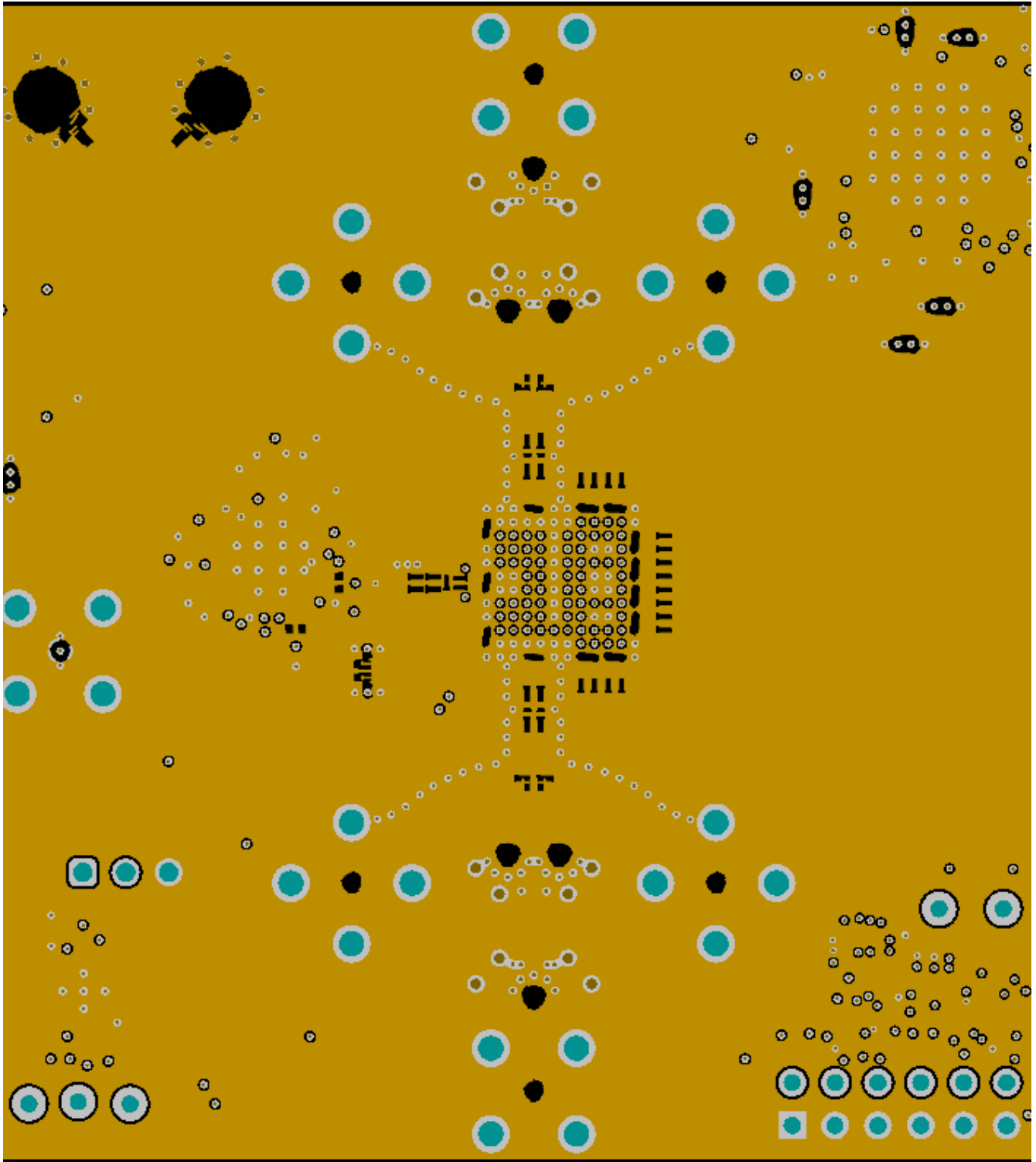
Figure 8-7. GND1 Cutouts to Optimize Impedance of Component Pads
