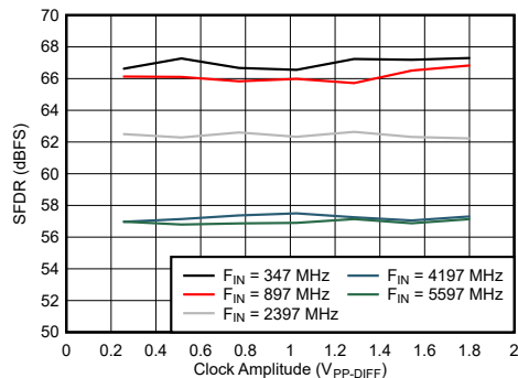
Figure 6-91. Dual Channel Mode: SFDR vs Clock Amplitude
