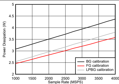
Figure 6-122. DES Mode: Power Dissipation vs Sample Rate
