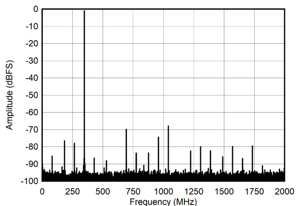
Figure 8-3. FFT for 347 MHz Input Signal, 4 GSPS, JMODE3
