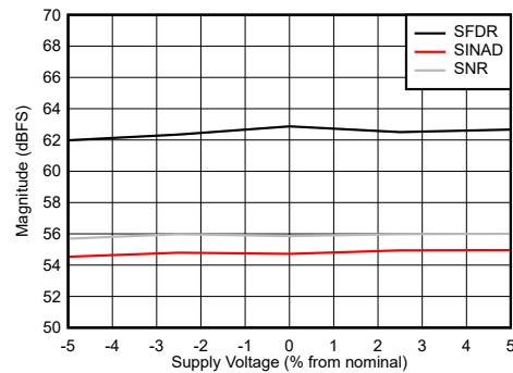
Figure 6-102. Dual Channel Mode: SNR, SINAD and SFDR vs Supply Voltage
