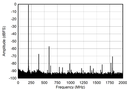
Figure 6-21. Dual Channel Mode: Single Tone FFT at 4197 MHz
