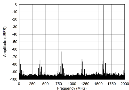
Figure 6-20. Dual Channel Mode: Single Tone FFT at 2397 MHz
