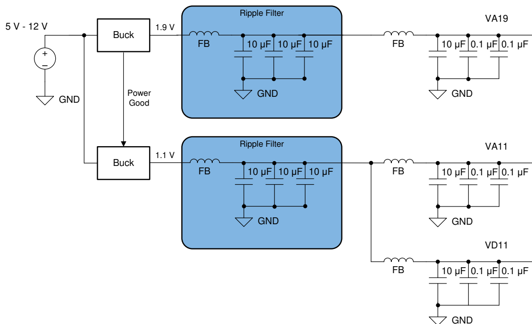
Figure 8-4. LDO Linear Regulator Approach Example
