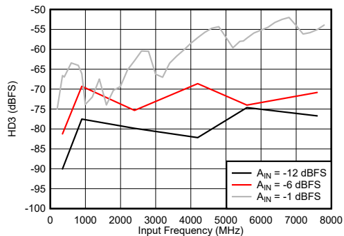
Figure 6-86. Dual Channel Mode: HD3 vs Input Frequency
