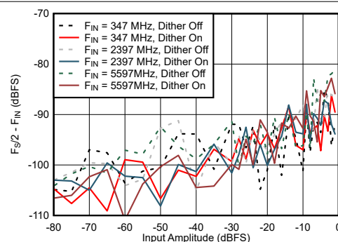
Figure 6-76. Dual Channel Mode: F_S/2 - F_{\text{IN}} vs Input Amplitude and Dither
