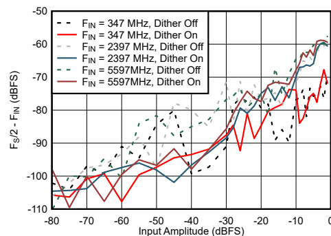
Figure 6-64. DES Mode: F_S/2 - F_{\text{IN}} vs Input Amplitude and Dither
