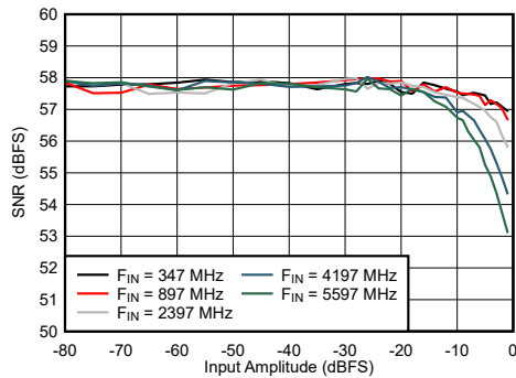
Figure 6-55. DES Mode: SNR vs Input Amplitude and Frequency
