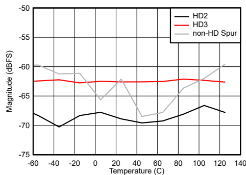
Figure 6-93. DES Mode: HD2, HD3 and Worst non-HD Spur vs Temperature
