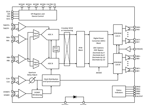
ADC12DJ4000RF Block Diagram
