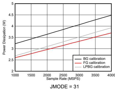
Figure 6-134. Dual Channel Mode: Power Dissipation vs Sample Rate
