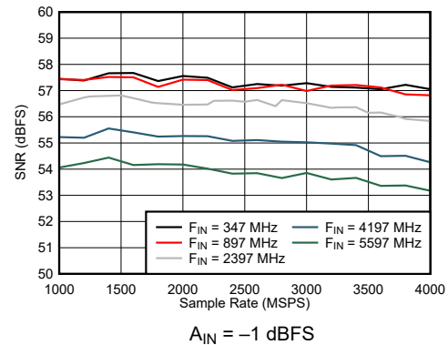
Figure 6-42. Dual Channel Mode: SNR vs Sample Rate and Input Frequency
