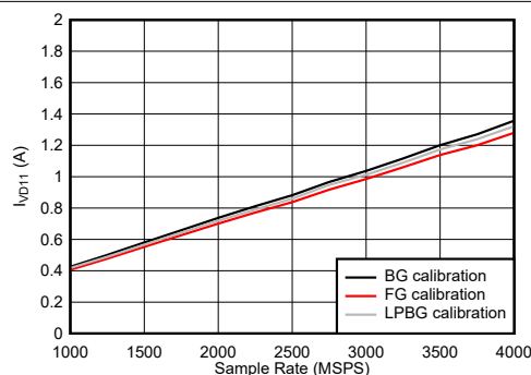
Figure 6-129. Dual Channel Mode: I_{VD11} vs Sample Rate
