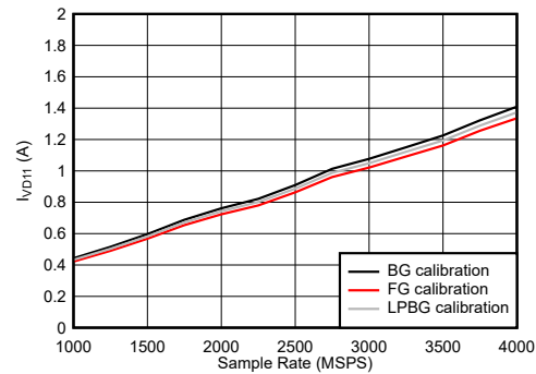
Figure 6-121. DES Mode: I_{VD11} vs Sample Rate
