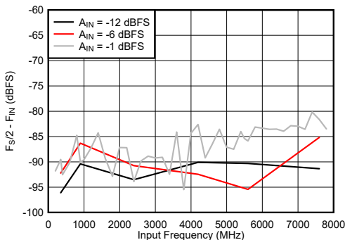
Figure 6-87. Dual Channel Mode: F_S/2 - F_{\text{IN}} vs Input Frequency
