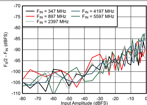
Figure 6-75. Dual Channel Mode: F_S/2 - F_{\text{IN}} vs Input Amplitude and Frequency
