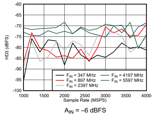
Figure 6-52. Dual Channel Mode: HD3 vs Sample Rate and Input Frequency
