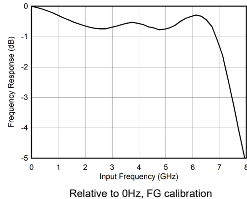
Figure 6-2. DES Mode: Input Response vs Input Frequency
