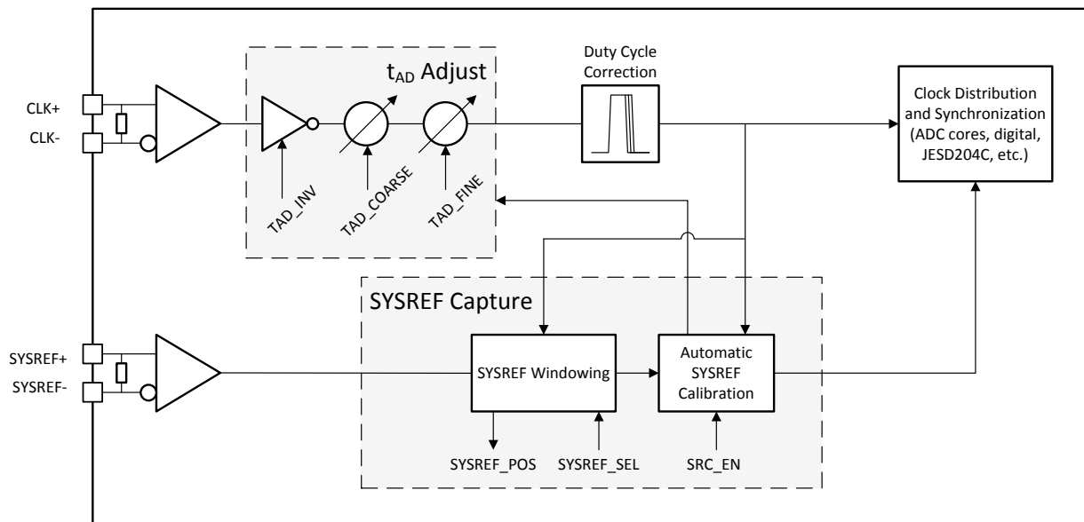
Figure 7-2. Clocking Subsystem
