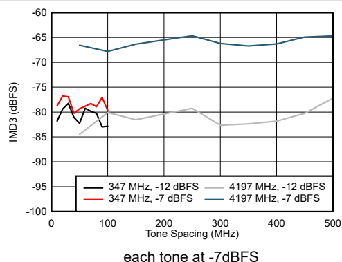
Figure 6-109. Dual Channel Mode: IMD3 vs Tone Spacing
