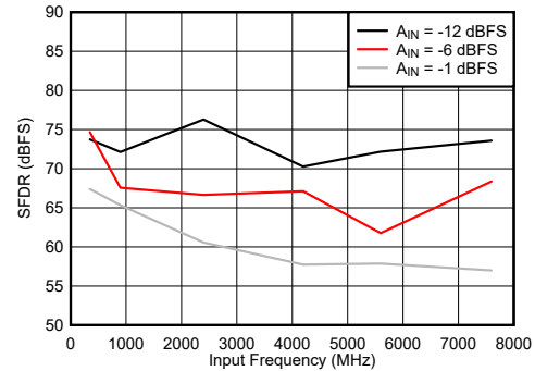
Figure 6-78. DES Mode: SFDR vs Input Frequency
