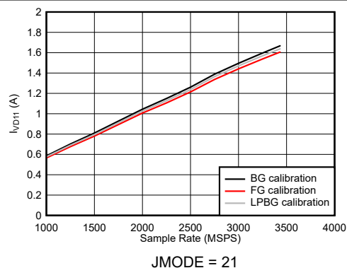
Figure 6-119. DES Mode: I_{VD11} vs Sample Rate
