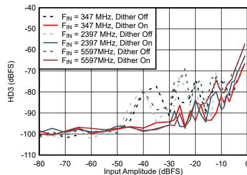
Figure 6-74. Dual Channel Mode: HD3 vs Input Amplitude and Dither
