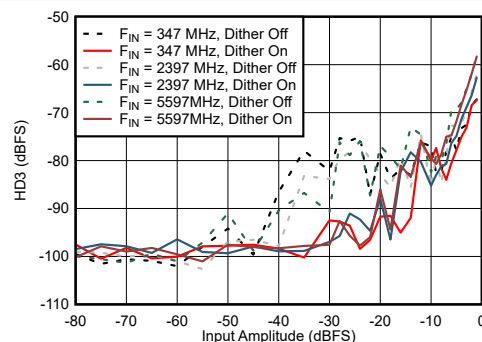
Figure 6-62. DES Mode: HD3 vs Input Amplitude and Dither
