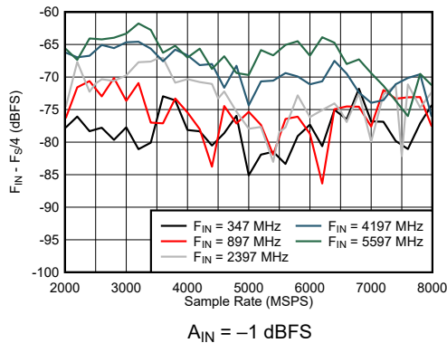
Figure 6-41. DES Mode: F_{\text{IN}} \pm F_{\text{S}}/4 vs Sample Rate and Input Frequency
