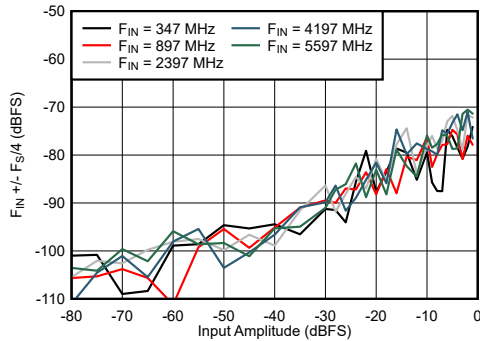
Figure 6-65. DES Mode: F_{\text{IN}} \pm F_{\text{IN}}/4 vs Input Amplitude and Frequency
