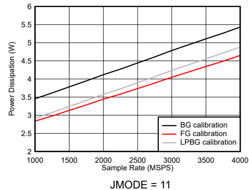
Figure 6-133. Dual Channel Mode: Power Dissipation vs Sample Rate
