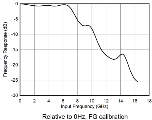
Figure 6-1. DES Mode: Input Amplitude vs Input Frequency
