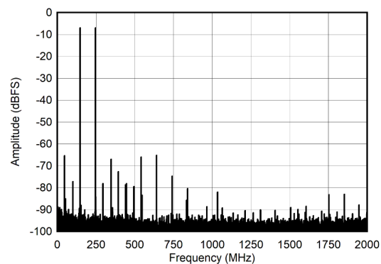
Figure 6-24. Dual Channel Mode: Two Tone FFT at 897 MHz
