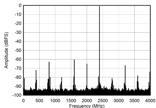
Figure 6-10. DES Mode: Single Tone FFT at 2397 MHz
