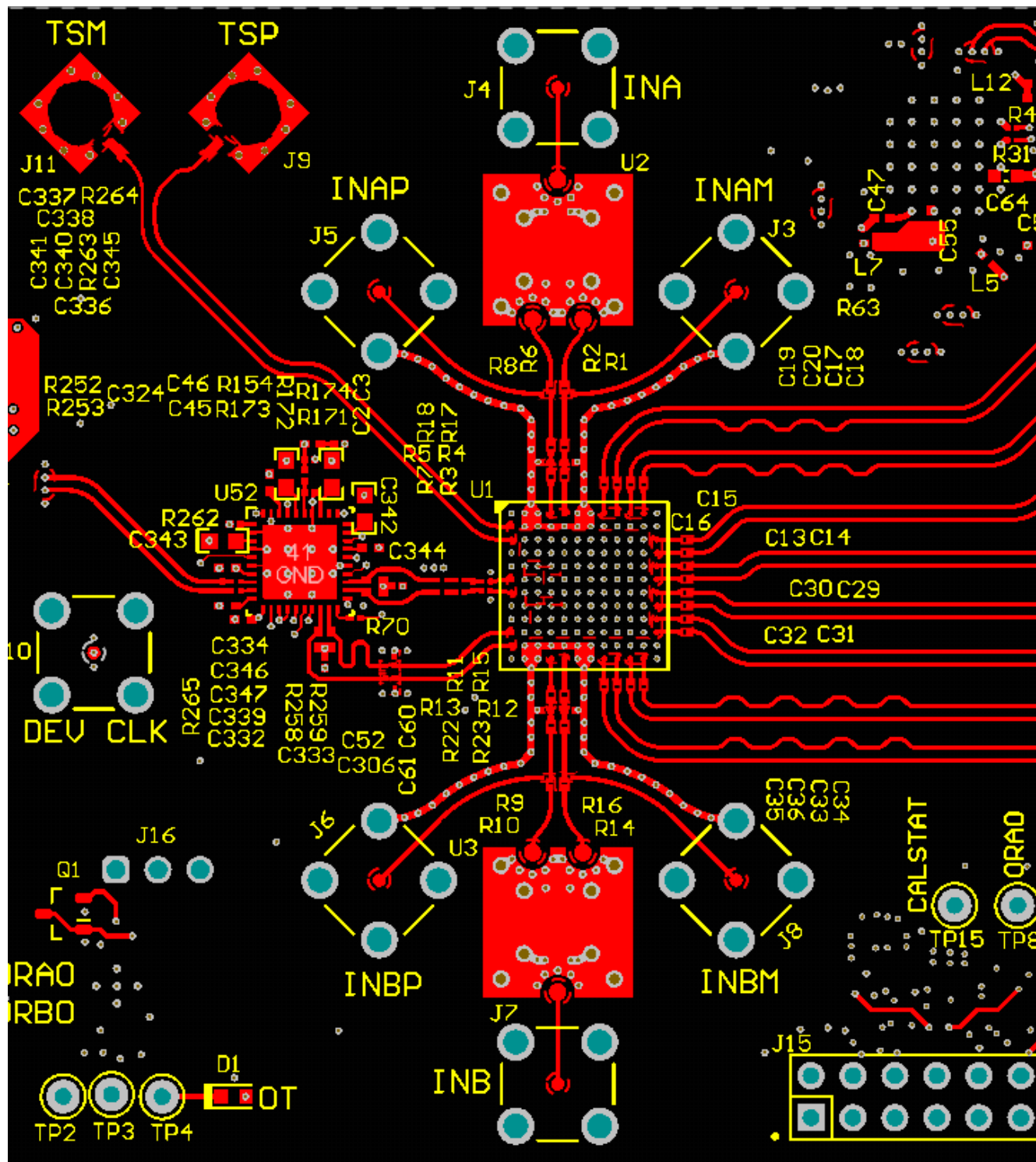
Figure 8-6. Top Layer Routing: Analog Inputs, CLK and SYSREF, DA0-3, DB0-3
