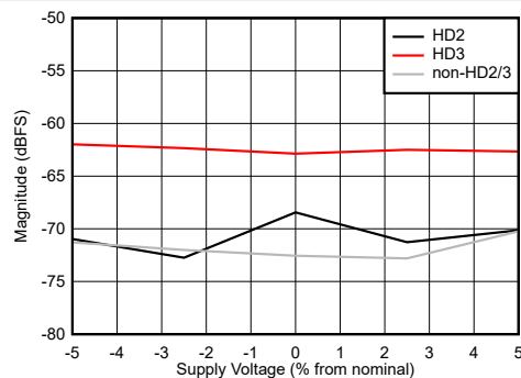
Figure 6-101. DES Mode: HD2, HD3 and Worst non-HD Spur vs Supply Voltage
