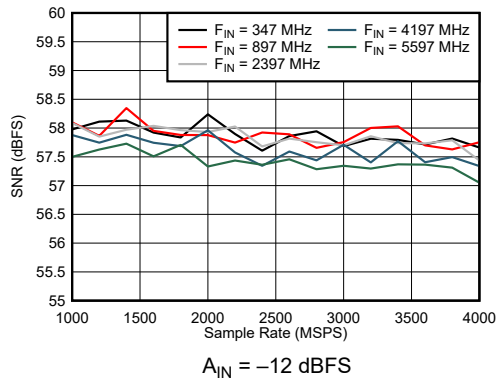
Figure 6-44. Dual Channel Mode: SNR vs Sample Rate and Input Frequency
