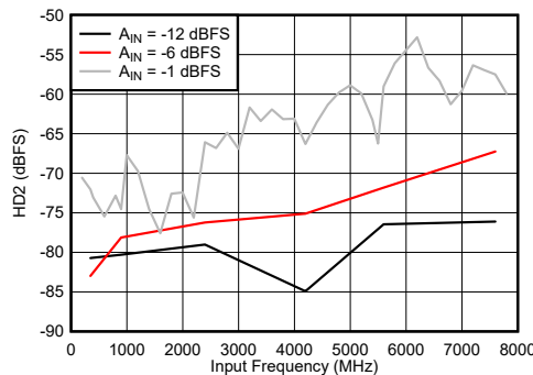
Figure 6-85. Dual Channel Mode: HD2 vs Input Frequency
