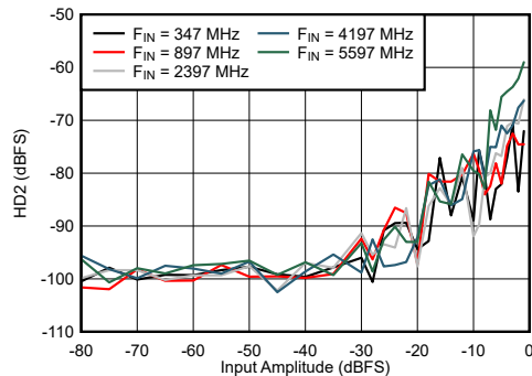
Figure 6-71. Dual Channel Mode: HD2 vs Input Amplitude and Frequency
