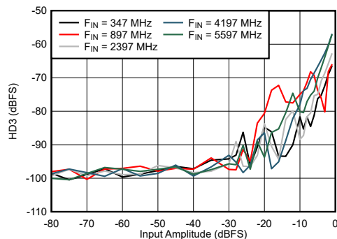
Figure 6-73. Dual Channel Mode: HD3 vs Input Amplitude and Frequency
