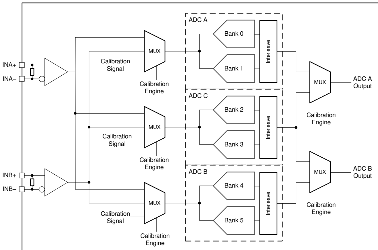
Figure 7-26. ADC12DJ4000RF Calibration System Block Diagram
