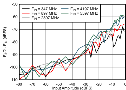
Figure 6-63. DES Mode: F_S/2 - F_{\text{IN}} vs Input Amplitude and Frequency
