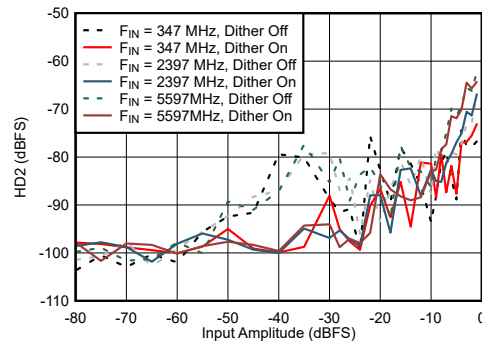
Figure 6-60. DES Mode: HD2 vs Input Amplitude and Dither
