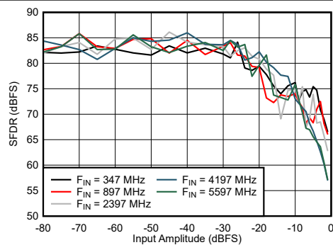
Figure 6-69. Dual Channel Mode: SFDR vs Input Amplitude and Frequency
