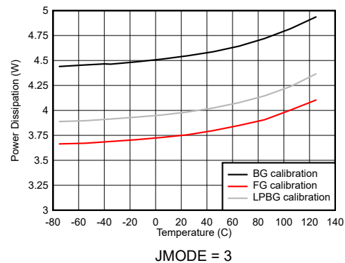
Figure 6-137. Dual Channel Mode: Power Dissipation vs Temperature
