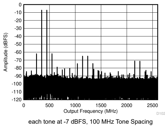
Figure 5-27. Dual Channel Mode: Two Tone FFT at 5597 MHz
