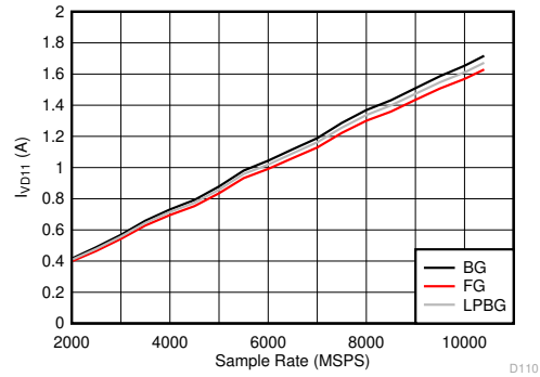
JMODE 61 Figure 5-128. DES Mode: I_{VD11} vs Sample Rate
