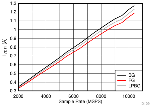
JMODE 30 Figure 5-127. DES Mode: I_{VD11} vs Sample Rate
