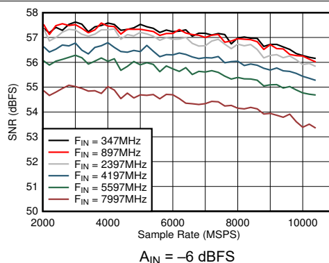
Figure 6-30. DES Mode: SNR vs Sample Rate and Input Frequency
