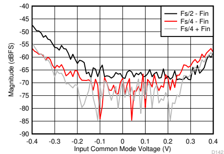
Figure 6-98. F_s/2 - F_{\text{IN}} and F_s/4 \pm F_{\text{IN}} vs Input Common Mode Voltage
