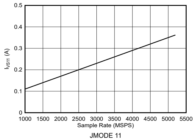
Figure 6-152. Dual Channel Mode: I_{VS11} vs Sample Rate (ADC12DJ5200RF)
