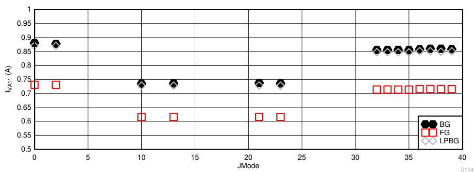
Figure 6-121. Other Modes with Lower Maximum F_S : I_{VA19} vs JMODE
