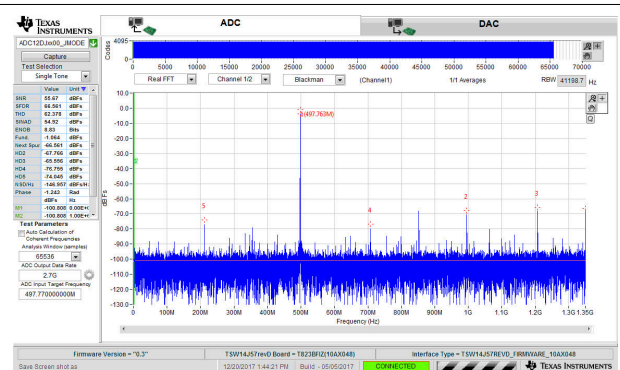
Figure 8-3. FFT for 497.77MHz Input Signal, 2.7GSPS, JMODE2
