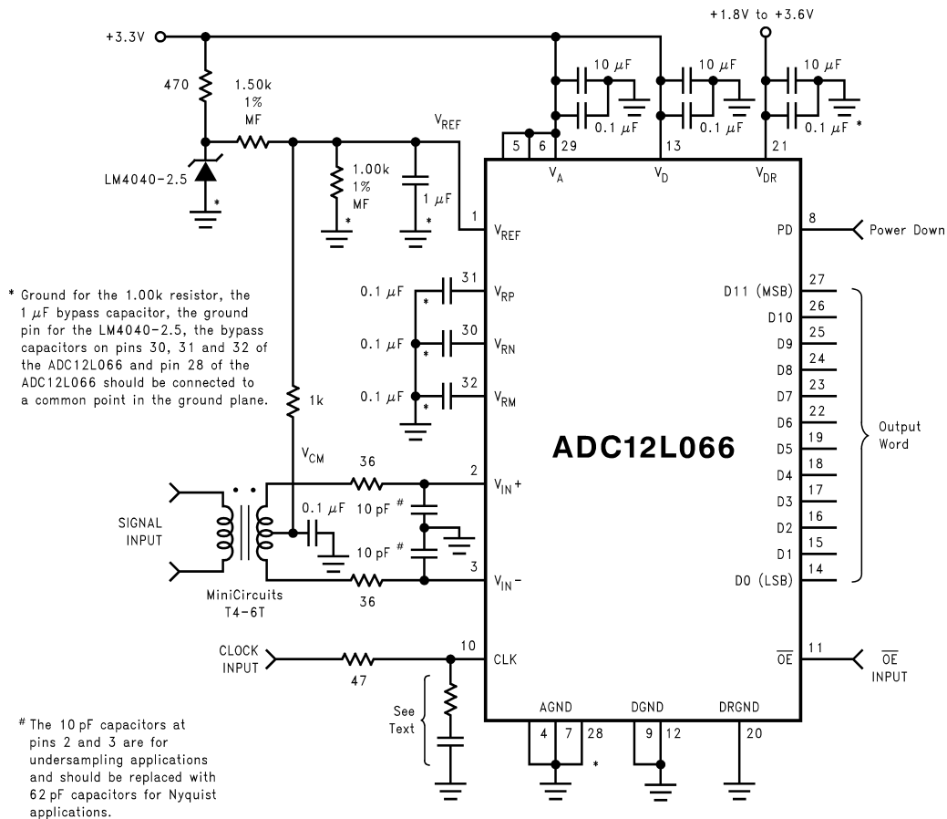
Figure 52. Driving the Signal Inputs with a Transformer
