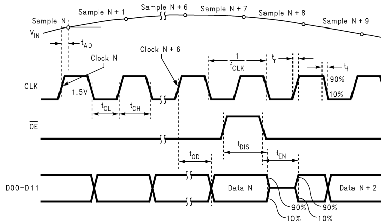
Figure 1. Output Timing
