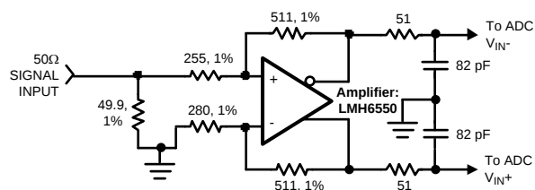
Figure 51. Differential Drive Circuit of Figure 50
