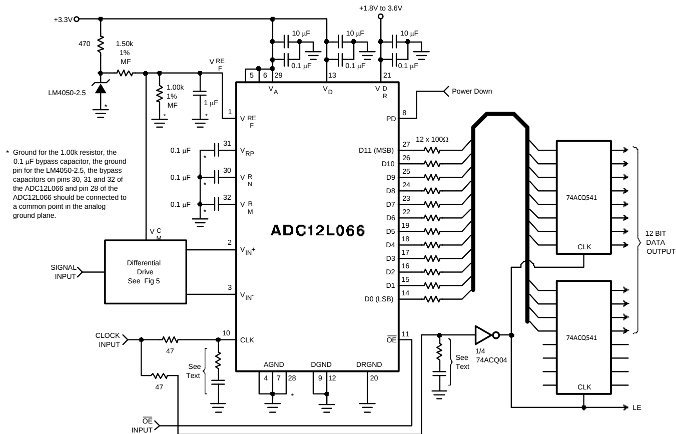
Figure 50. Simple Application Circuit with Single-Ended to Differential Buffer
