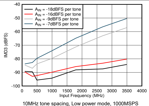
Figure 5-76. IMD3 vs F_{IN}
