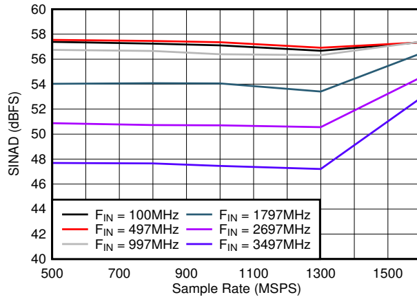
Figure 5-25. SINAD vs Sample Rate
