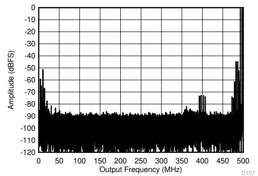
Figure 5-74. Two Tone FFT at 3498 MHz 10 MHz tone spacing, -7 dBFS per tone, Low power mode, 1000MSPS
