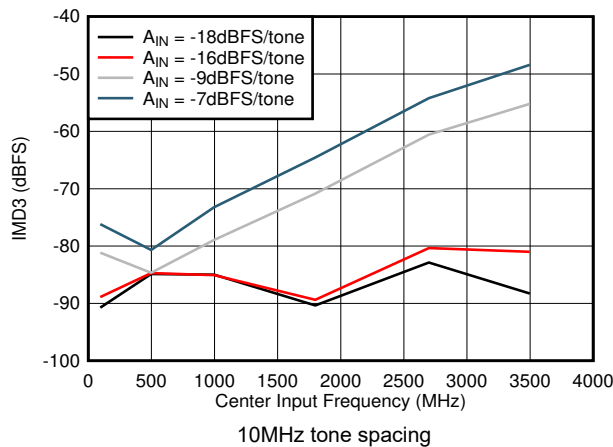
Figure 5-75. IMD3 vs F_{IN} 10MHz tone spacing
