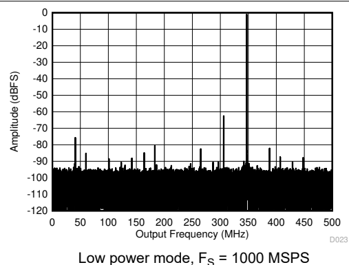
Figure 5-12. Single Tone FFT at 347 MHz and -1 dBFS
