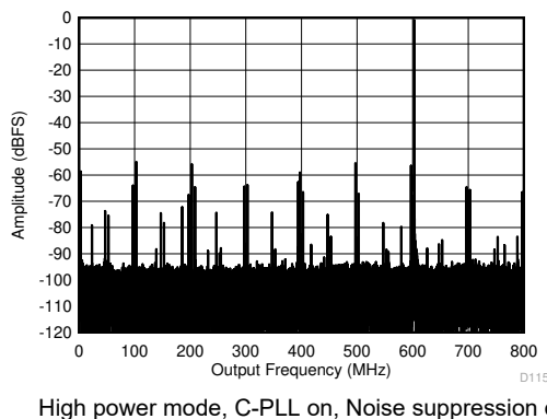
Figure 5-9. Single Tone FFT at 997 MHz and -1 dBFS
