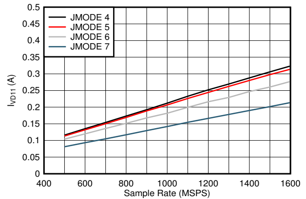
Figure 5-106. Single Channel, I_{VD11} vs F_S and JMODE 4 - 7
