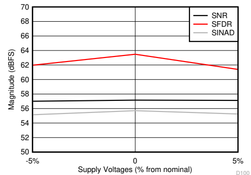
Figure 5-60. SNR, SFDR and SINAD vs Supply Voltage
