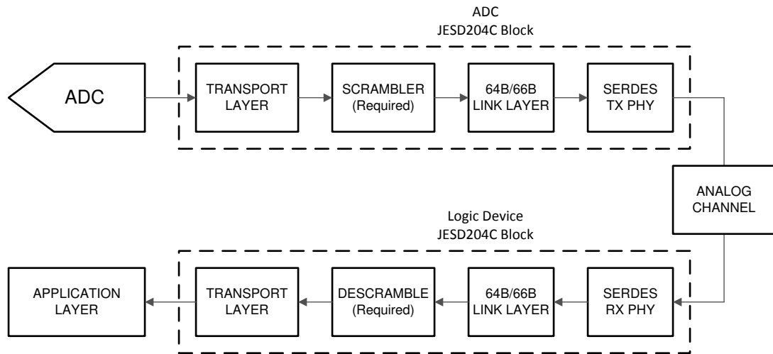
Figure 6-6. Simplified 64B/66B Encoded JESD204C Interface Diagram
