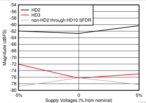
Figure 5-61. HD2, HD3 and Worst non-HD Spur vs Supply Voltage
