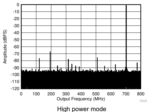
Figure 5-7. Single Tone FFT at 847 MHz and -1 dBFS
