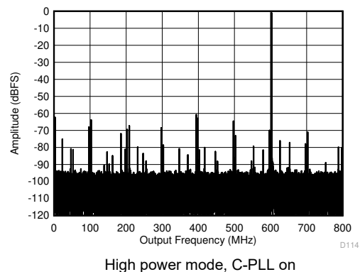
Figure 5-8. Single Tone FFT at 997 MHz and -1 dBFS
