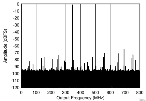
Figure 5-5. Single Tone FFT at 347 MHz and -1 dBFS
