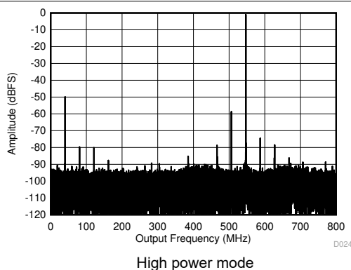
Figure 5-11. Single Tone FFT at 3797 MHz and -1 dBFS
