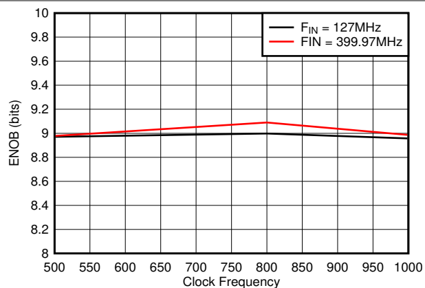
Low power mode Figure 5-31. ENOB vs Sample Rate
