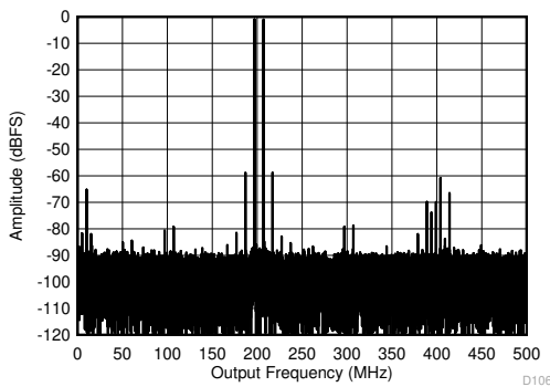
Figure 5-73. Two Tone FFT at 1798 MHz 10 MHz tone spacing, -7 dBFS per tone, Low power mode, 1000MSPS
