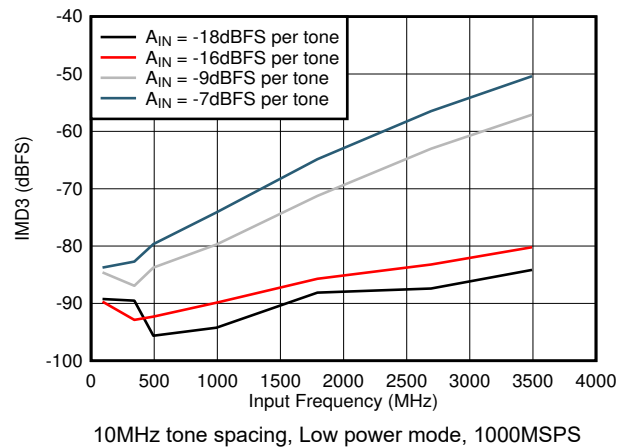
Figure 5-76. IMD3 vs F_{IN} 10MHz tone spacing, Low power mode, 1000MSPS
