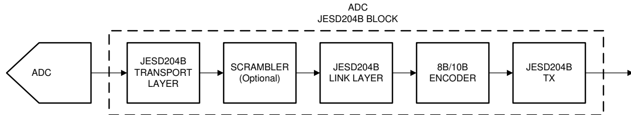
Figure 6-41. JESD204B Block Diagram
