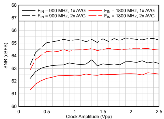
Figure 6-13. SNR vs Clock Amplitude (Dither ON)
