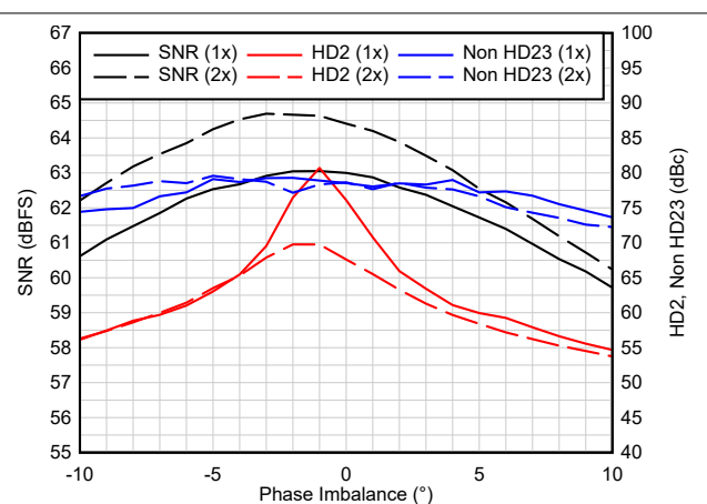
Figure 6-4. Phase Imbalance - 2.6 GSPS
