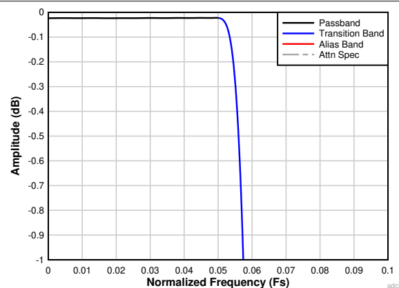
Figure 6-27. Decimation by 8 Passband Ripple Response
