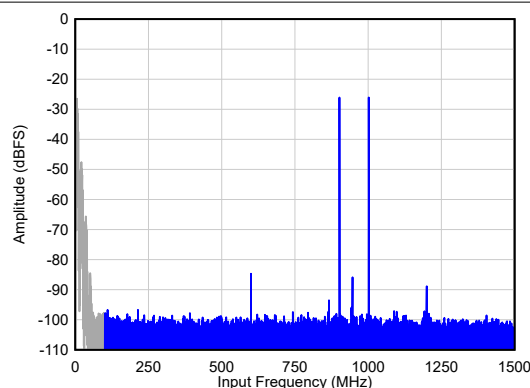
IMD3 = 71 dBc A_{IN} = -26\text{ dBFS/tone} , 1x AVG, Dither = EN Figure 5-22. Two Tone FFT at F_{IN} = 900/1000\text{ MHz}
