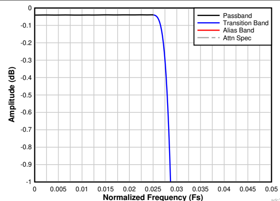
Figure 6-29. Decimation by 16 Passband Ripple Response
