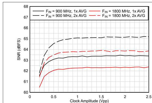
Figure 6-12. SNR vs Clock Amplitude (Dither OFF)
