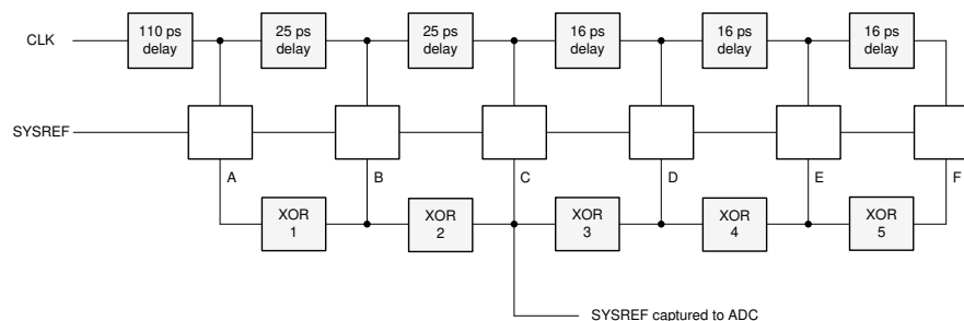
Figure 6-21. SYSREF Detection Circuitry
