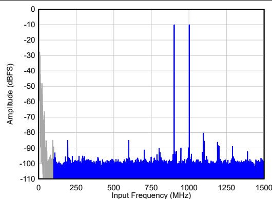
IMD3 = 70 dBc A_{IN} = -10\text{ dBFS/tone} , 1x AVG, Dither = EN Figure 5-20. Two Tone FFT at F_{IN} = 900/1000\text{ MHz}
