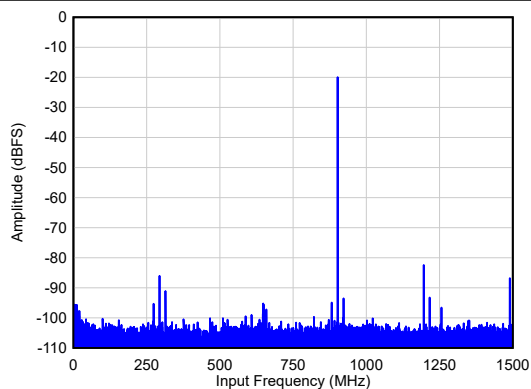
Figure 5-15. Single Tone FFT at F_{IN} = 900 MHz
