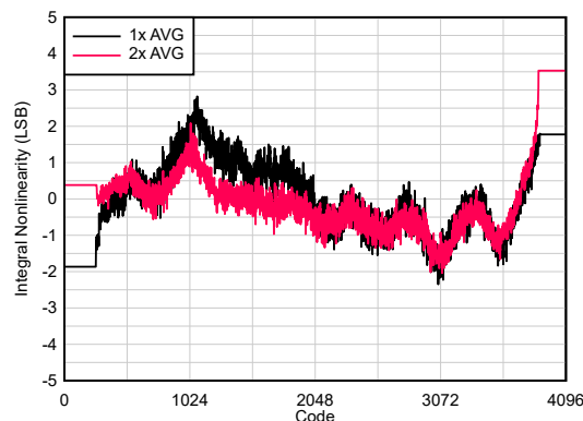
Figure 5-38. INL vs Code
