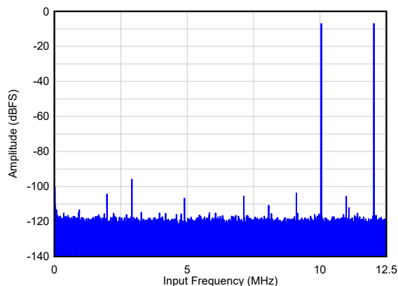
A_{IN} = -7 dBFS/tone, IMD3 = 100 dBc Figure 6-24. Two Tone FFT at F_{IN} = 10, 12 MHz
