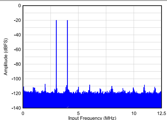
Figure 6-23. Two Tone FFT at F_{IN} = 3, 4\text{ MHz}
