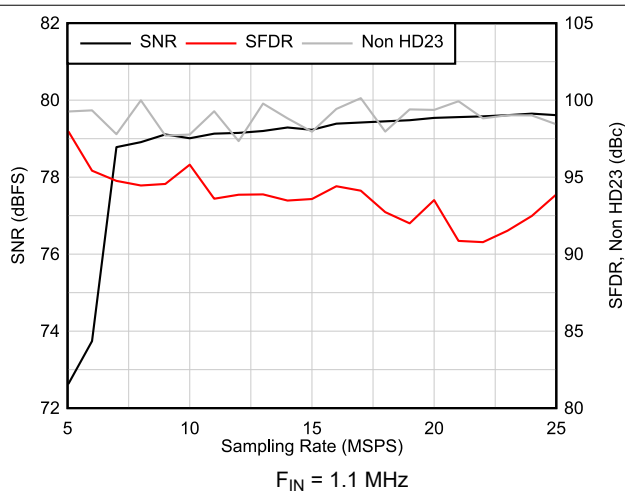
F_{IN} = 1.1 MHz Figure 6-28. AC Performance vs Sampling Rate
