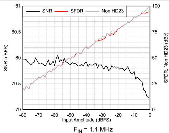
Figure 6-6. AC Performance vs Input Amplitude
