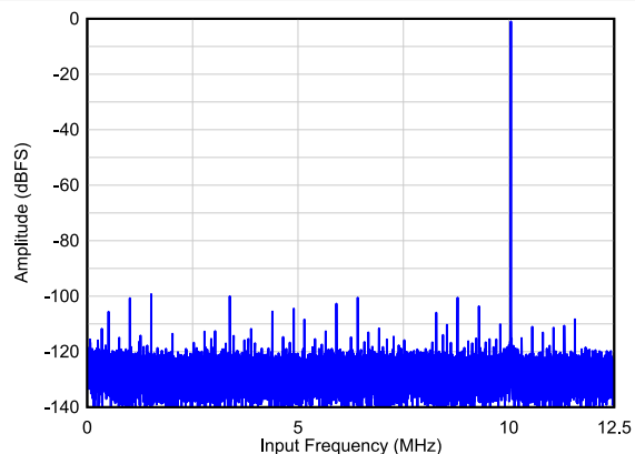
Figure 6-19. Single Tone FFT at F_{IN} = 10\text{ MHz}
