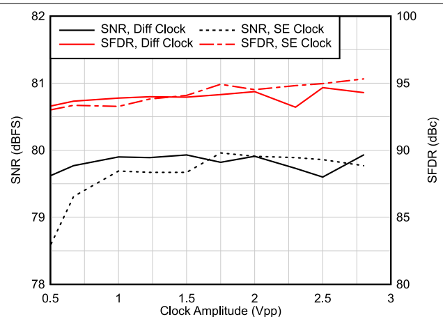
Differential (Diff) vs Single ended (SE) clock, F_{IN} = 5 MHz Figure 6-29. AC Performance vs Clock Amplitude
