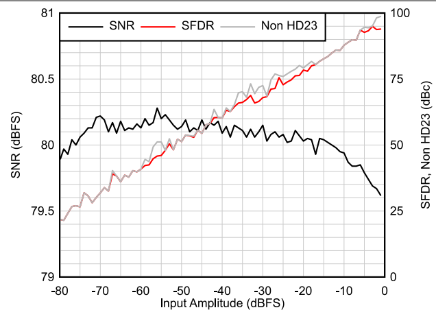
F_{IN} = 5 MHz Figure 6-27. AC Performance vs Input Amplitude
