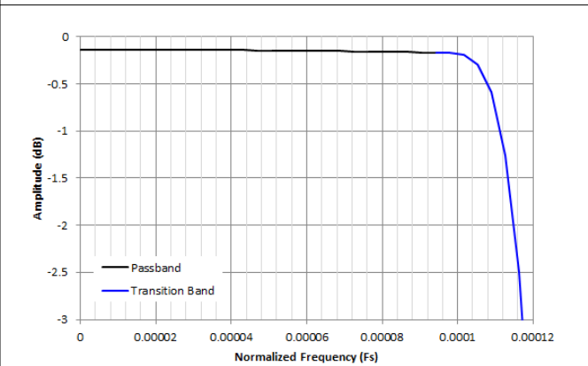
Figure 8-47. Decimation by 4096 Passband Ripple Response
