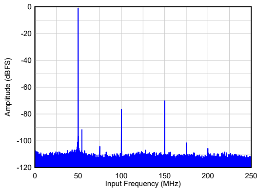
SNR = 70.7dBFS, HD23 = 74dBc, Non HD23 = 92dBFS
