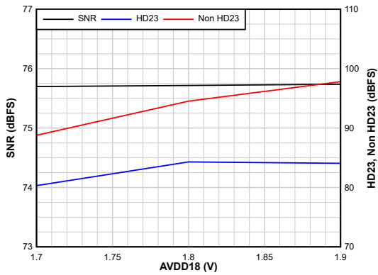
Figure 6-19. AC Performance vs AVDD18
