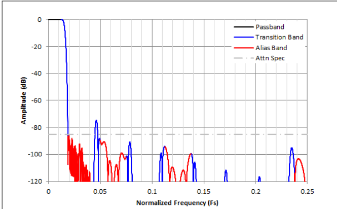
Figure 8-32. Complex Decimation by 32 Filter Response
