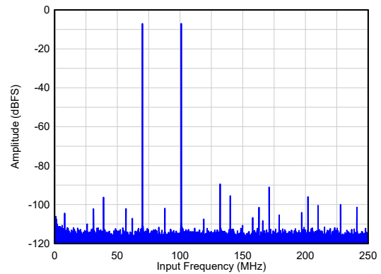
A_{IN} = -7\text{dBFS}/\text{tone} , IMD3 = 84dBc
