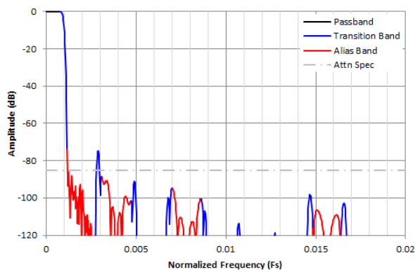
Figure 8-40. Complex Decimation by 512 Filter Response
