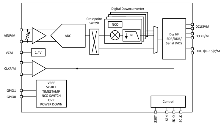
Block Diagram
