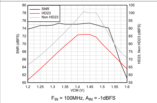
Figure 6-48. AC Performance vs VCM
