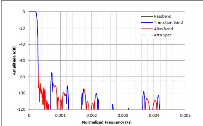
Figure 8-44. Complex Decimation by 2048 Filter Response
