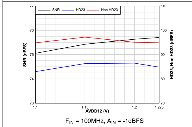
Figure 6-47. AC Performance vs AVDD12
