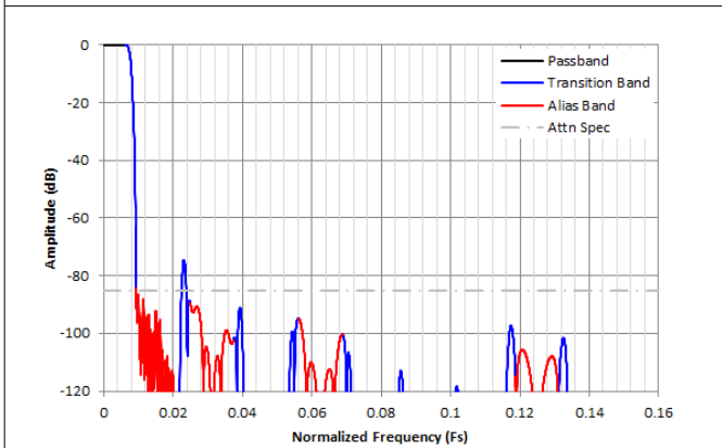
Figure 8-34. Complex Decimation by 64 Filter Response
