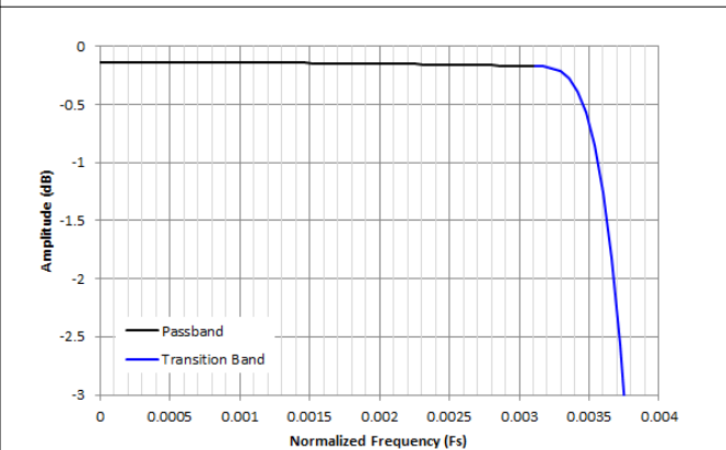
Figure 8-37. Decimation by 128 Passband Ripple Response
