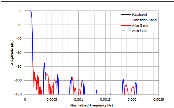
Figure 8-46. Complex Decimation by 4096 Filter Response
