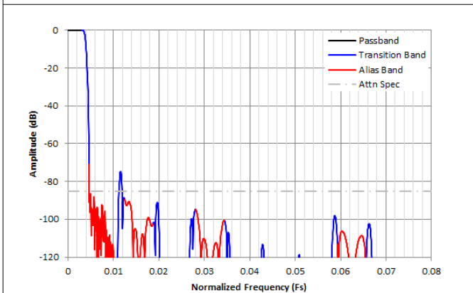
Figure 8-36. Complex Decimation by 128 Filter Response
