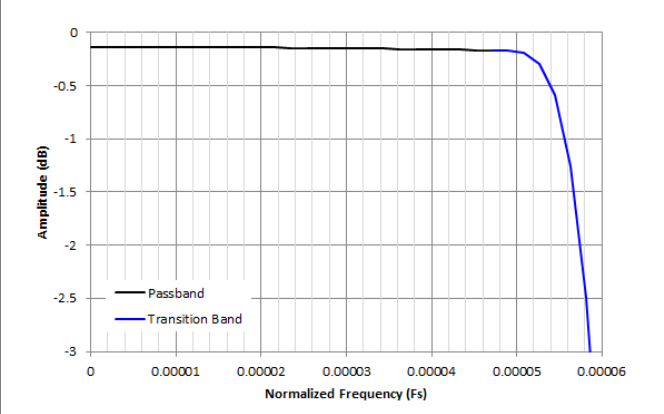
Figure 8-49. Decimation by 8192 Passband Ripple Response
