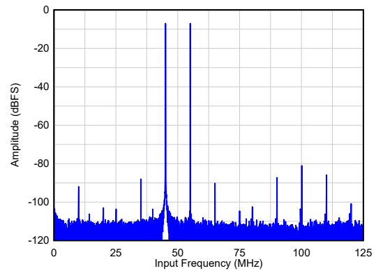
A_{IN} = -7\text{dBFS}/\text{tone} , IMD3 = 81dBc
