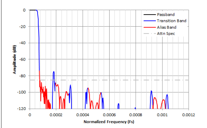
Figure 8-48. Complex Decimation by 8192 Filter Response
