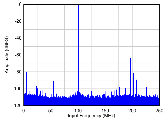
SNR = 68.9dBFS, HD23 = 69dBc, Non HD23 = 81dBFS
