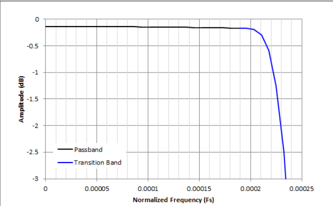
Figure 8-45. Decimation by 2048 Passband Ripple Response
