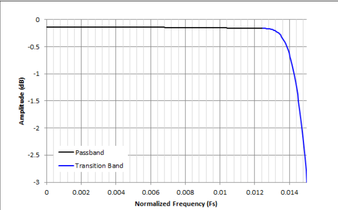
Figure 8-33. Decimation by 32 Passband Ripple Response
