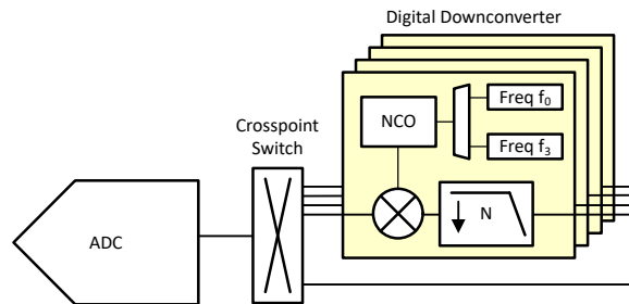
Figure 8-21. Internal digital down converter
