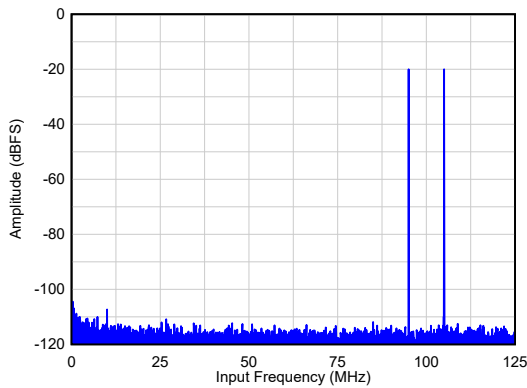
A_{IN} = -20\text{dBFS}/\text{tone} , IMD3 = 92dBc
