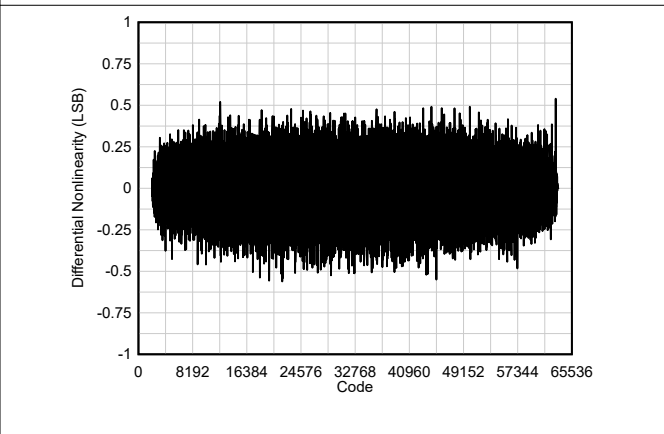
Figure 6-50. DNL
