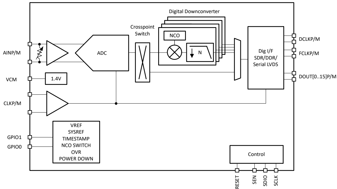
Figure 8-1. Block Diagram
