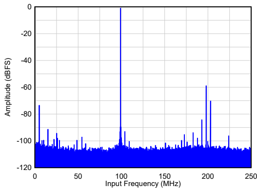
SNR = 65.7dBFS, HD23 = 63dBc, Non HD23 = 74dBFS
