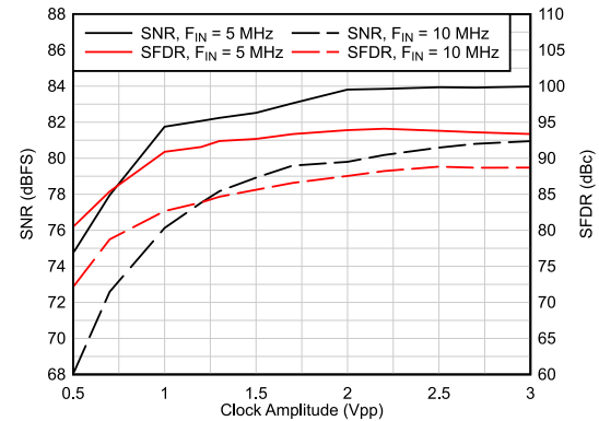
Figure 5-16. AC Performance vs Clock Amplitude Single ended clock input
