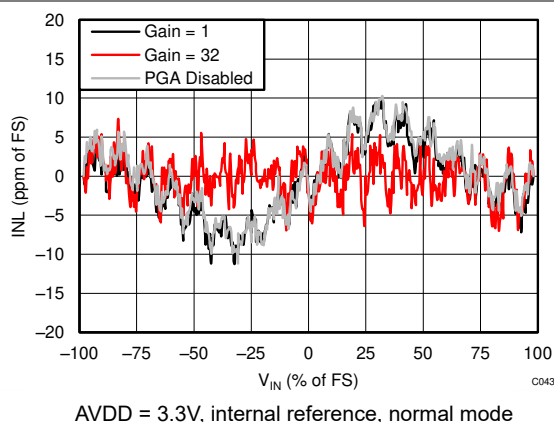
Figure 6-9. Integral Nonlinearity vs Differential Input Signal
