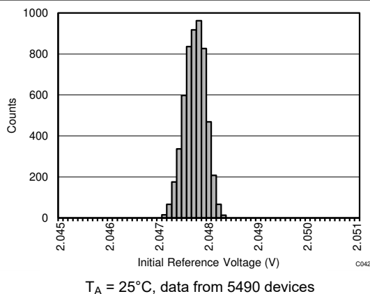
Figure 6-11. Internal Reference Voltage Histogram
