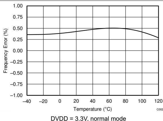
Figure 6-13. Internal Oscillator Accuracy vs Temperature
