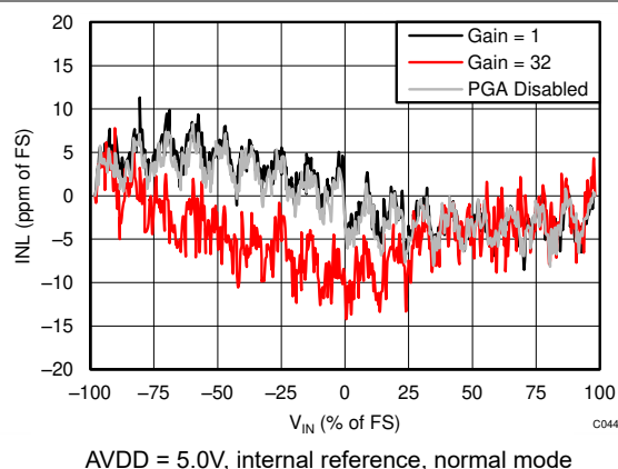
Figure 6-10. Integral Nonlinearity vs Differential Input Signal
