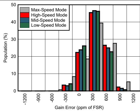
Figure 5-16. Gain Error Histograms
