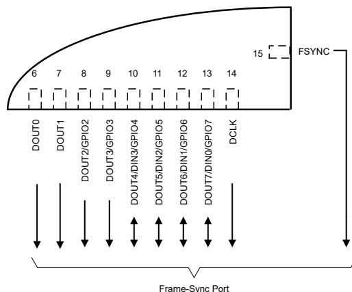
Figure 7-30. ADS117L18 Frame-Sync Port Pins
