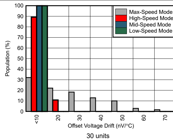
Figure 5-15. Offset Voltage Drift Histograms
