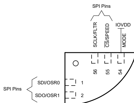
Figure 7-45. SPI Pins
