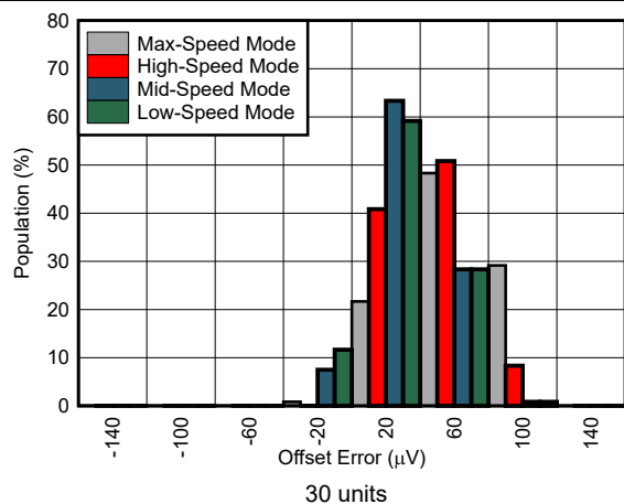
Figure 5-14. Offset Voltage Histograms
